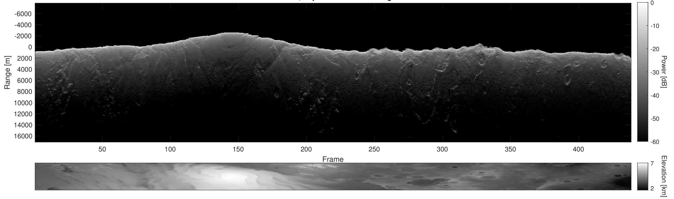
Orbit 23171, Depth-Corrected Cluttergram
