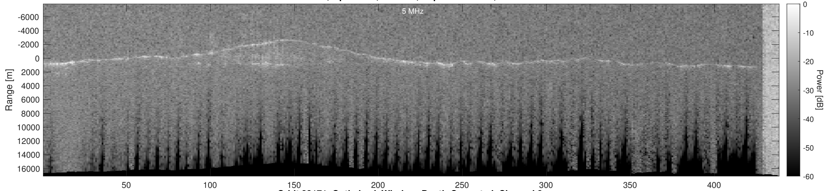
Orbit 23171, Optimized, Window, Depth-Corrected, Channel 2
