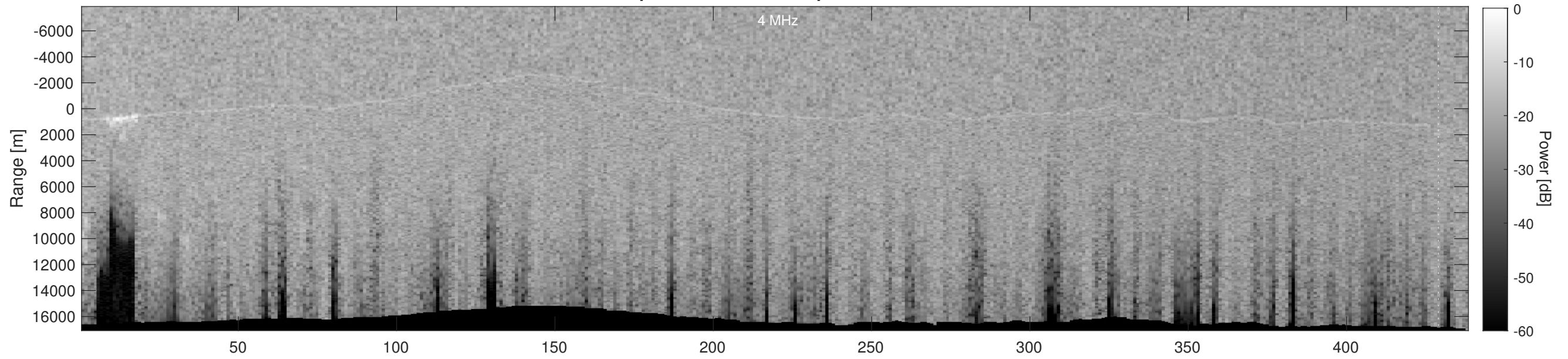
Orbit 23171, Depth-Corrected Cluttergram
