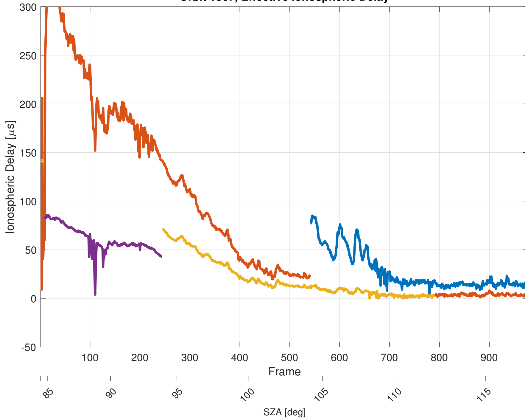
Orbit 1867, Effective Ionospheric Delay
