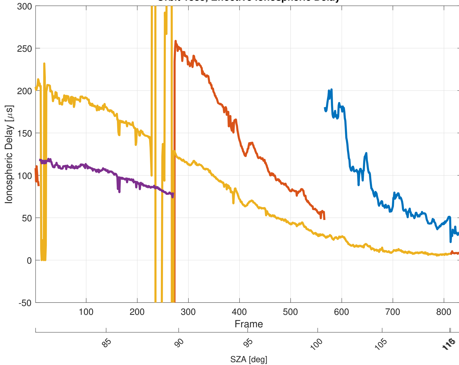
Orbit 1883, Effective Ionospheric Delay
