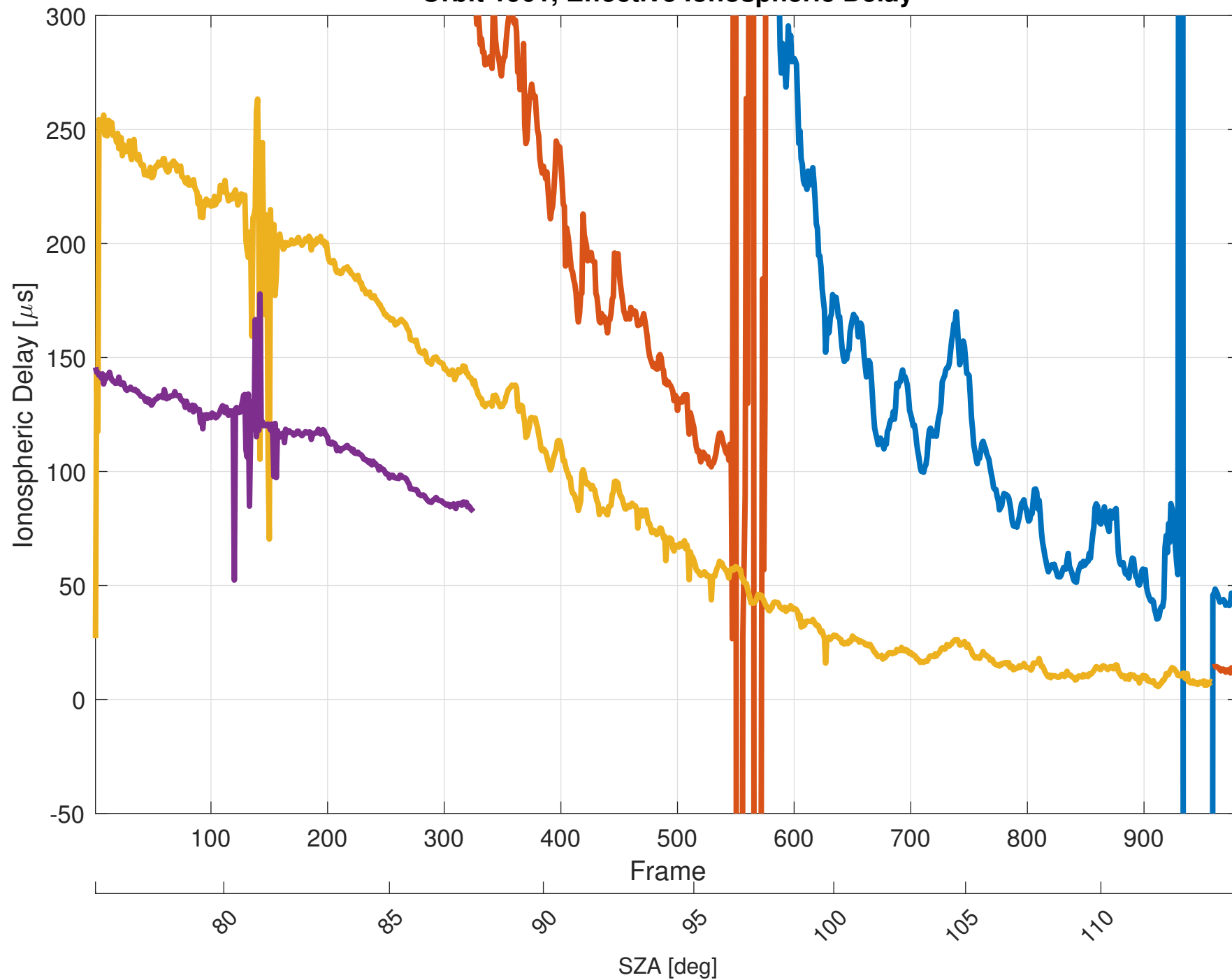
Orbit 1901, Effective Ionospheric Delay
