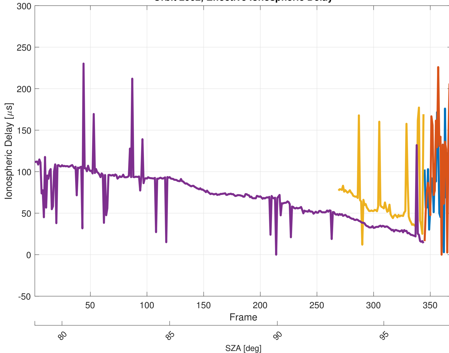
Orbit 2002, Effective Ionospheric Delay
