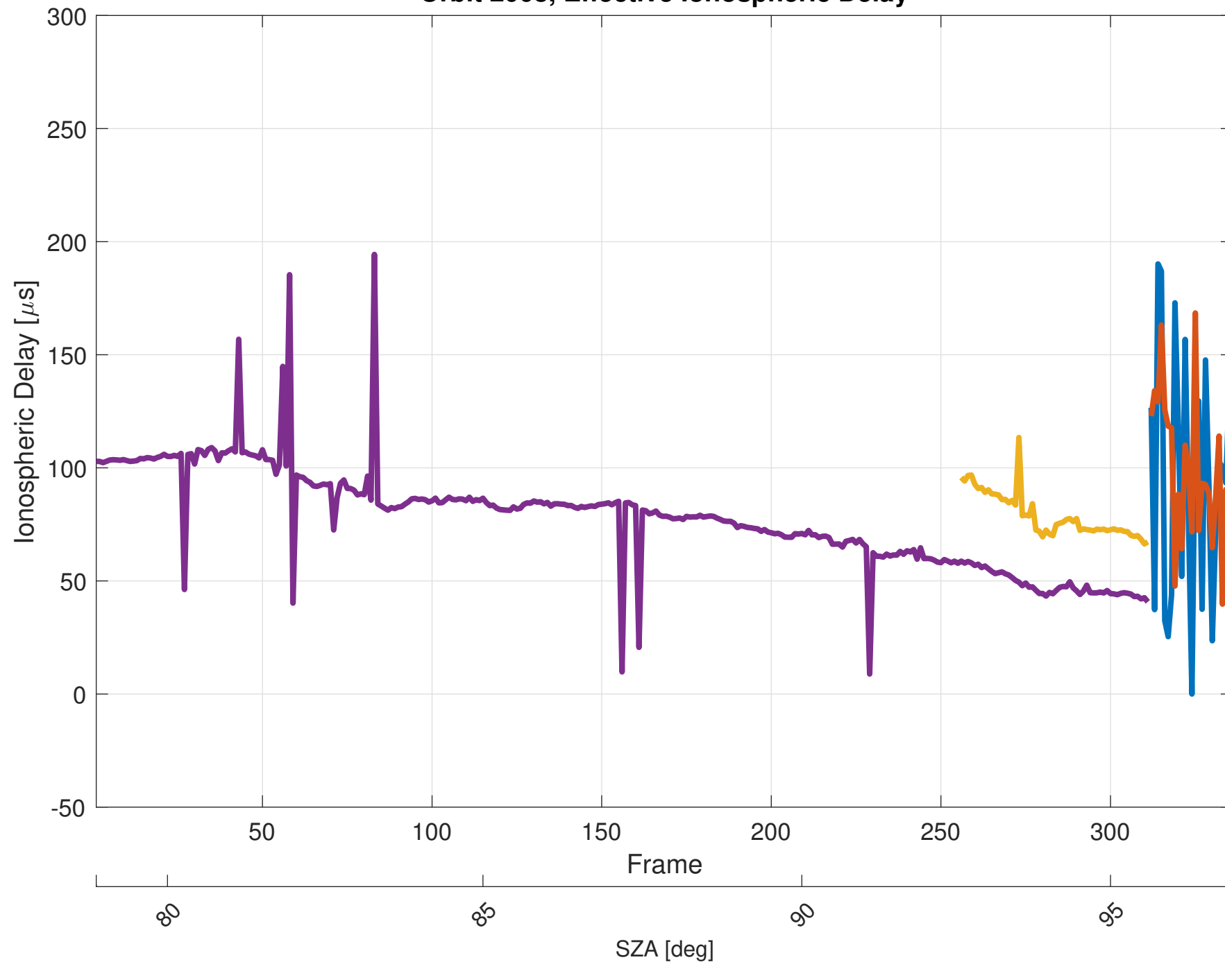
Orbit 2008, Effective Ionospheric Delay
