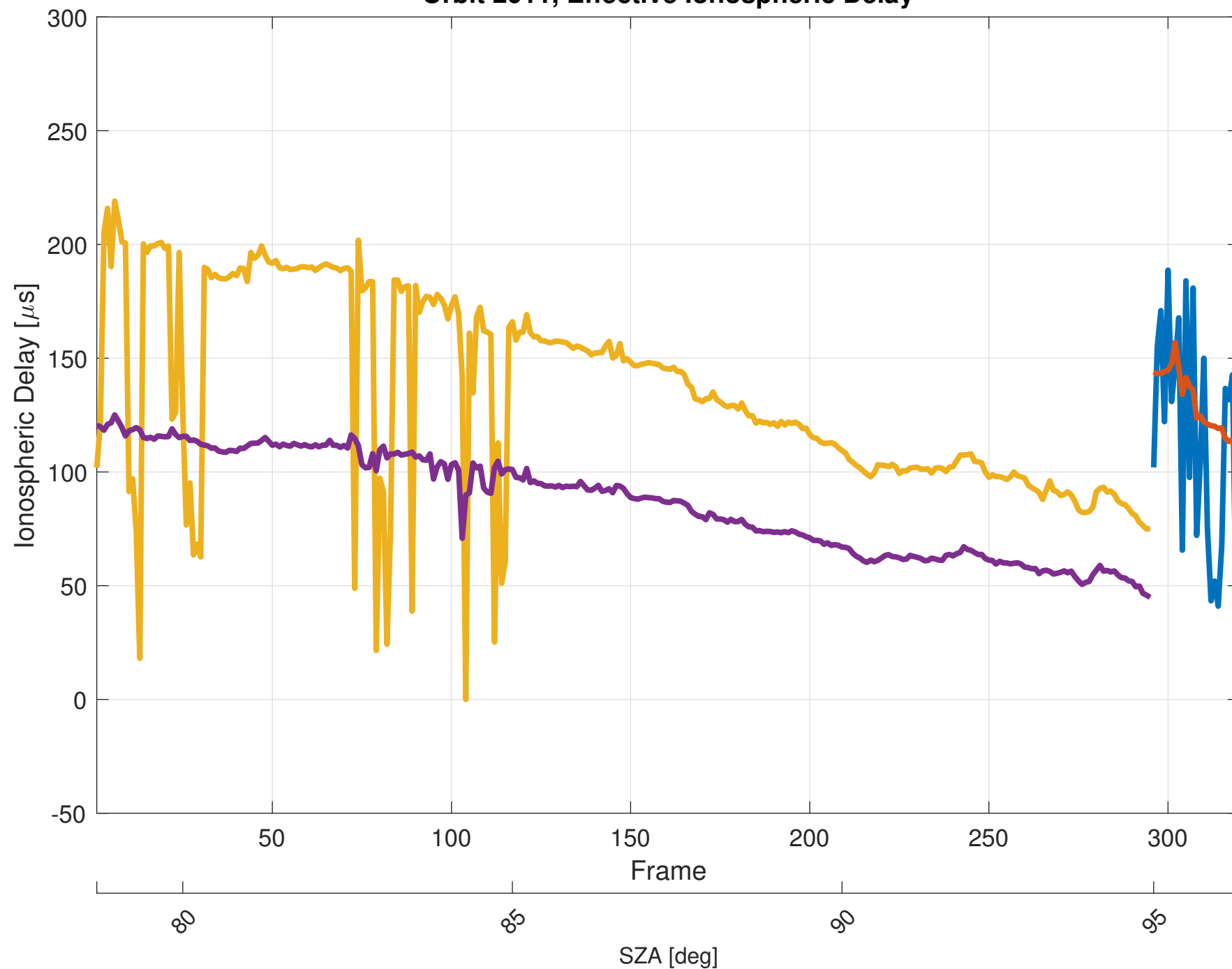
Orbit 2011, Effective Ionospheric Delay
