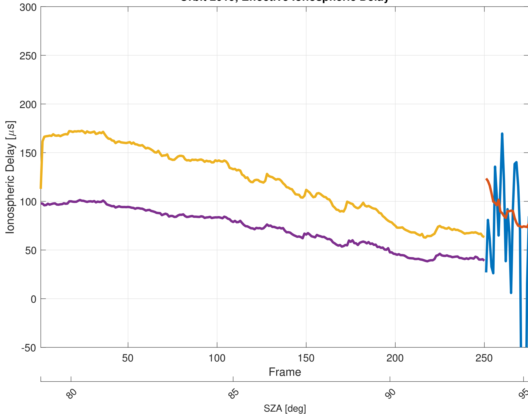
Orbit 2019, Effective Ionospheric Delay
