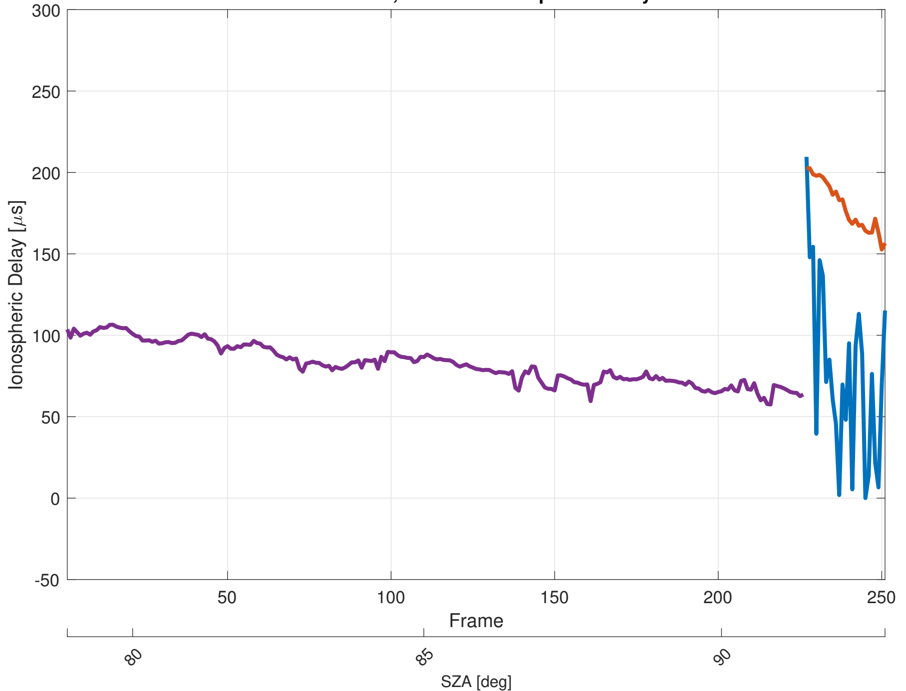
Orbit 2027, Effective Ionospheric Delay
