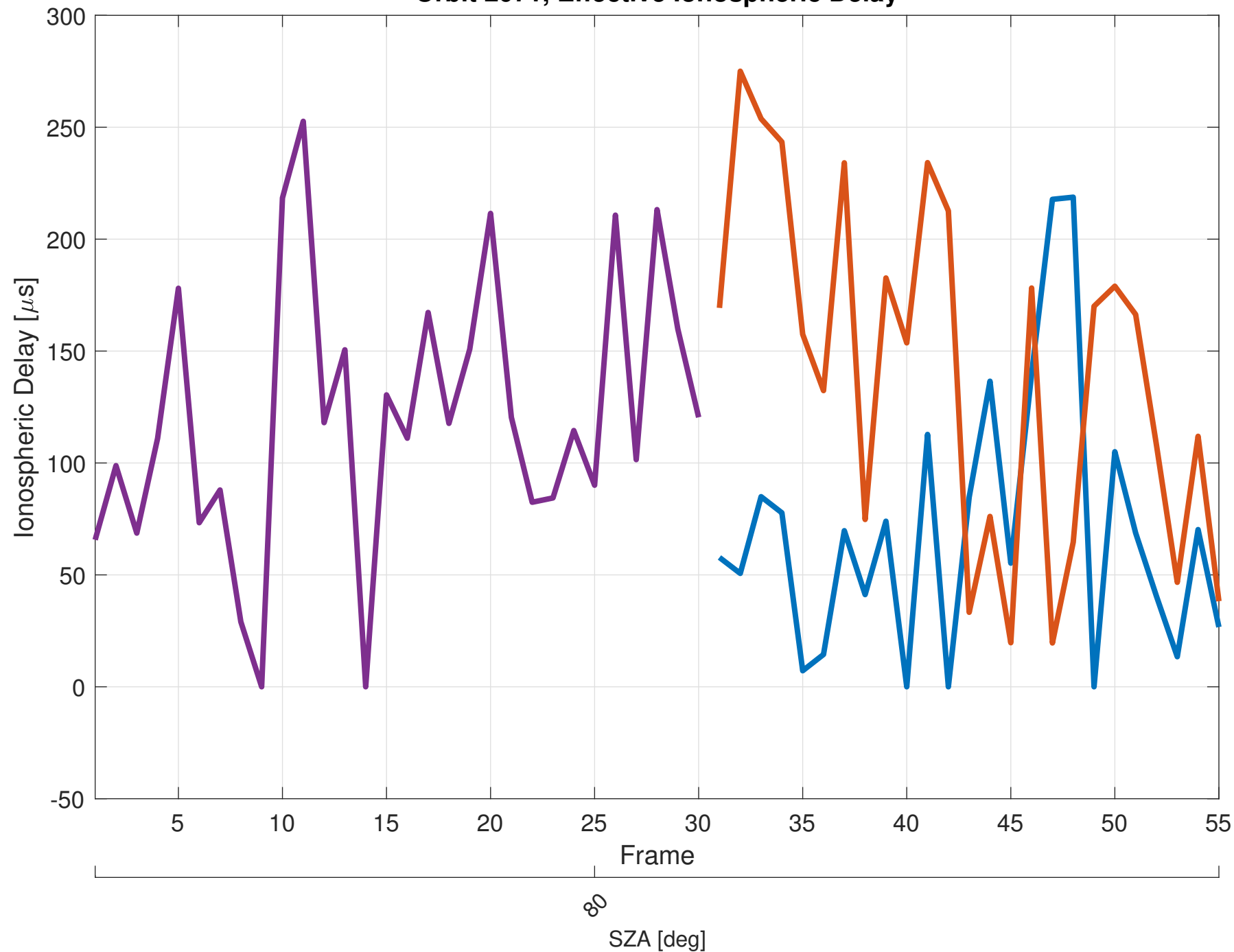
Orbit 2071, Effective Ionospheric Delay
