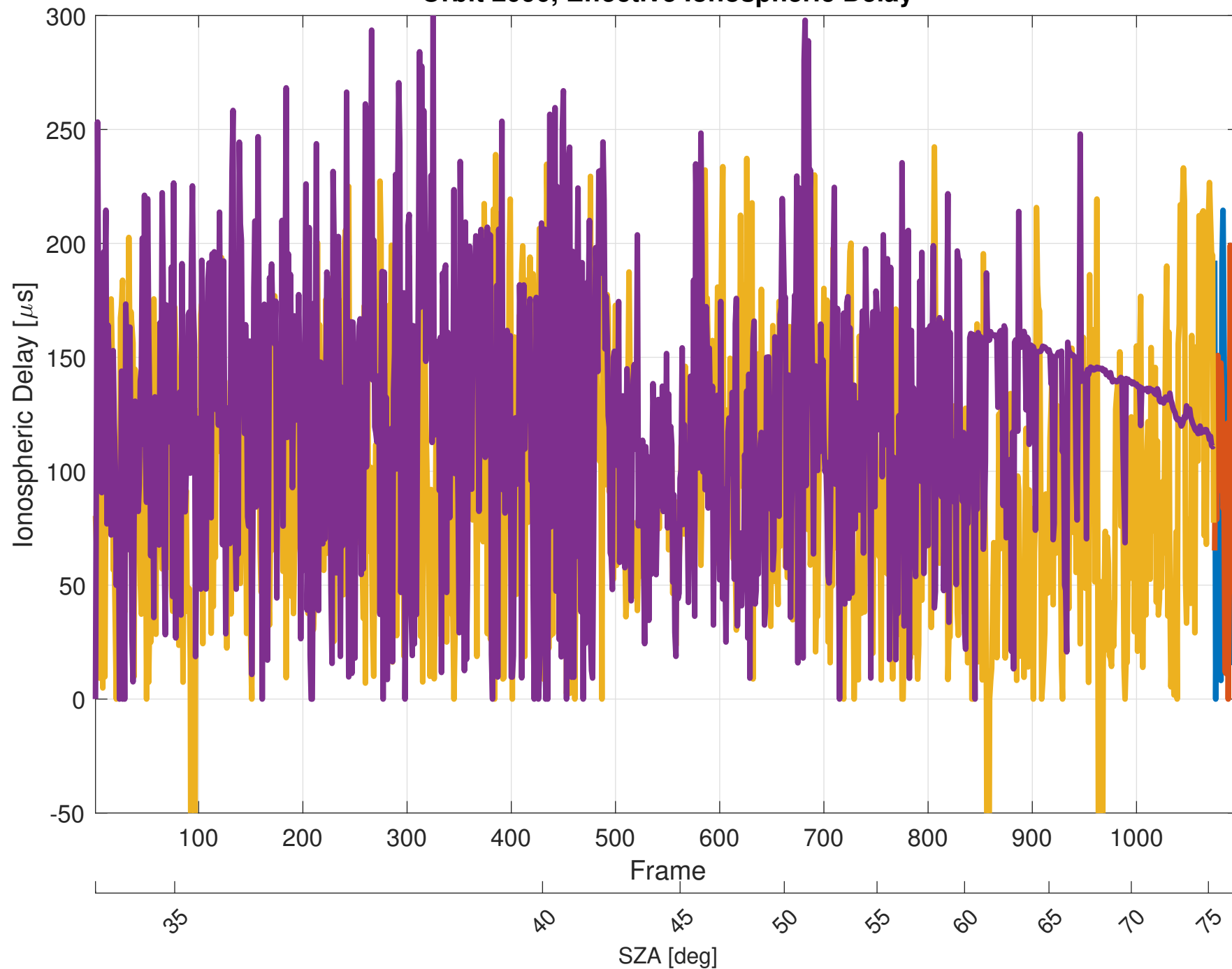
Orbit 2090, Effective Ionospheric Delay
