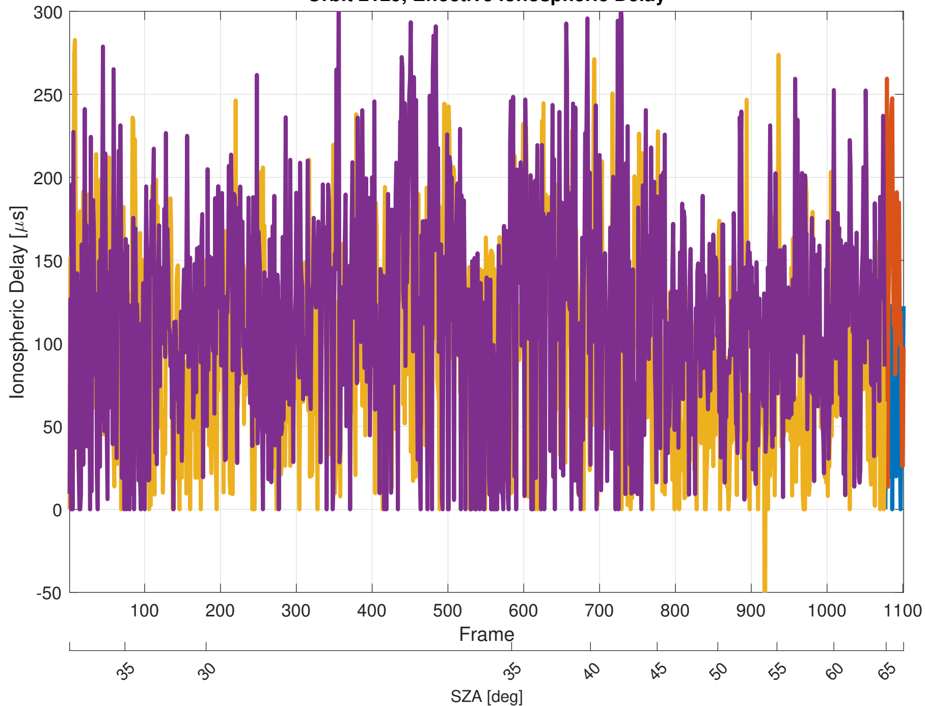
Orbit 2129, Effective Ionospheric Delay
