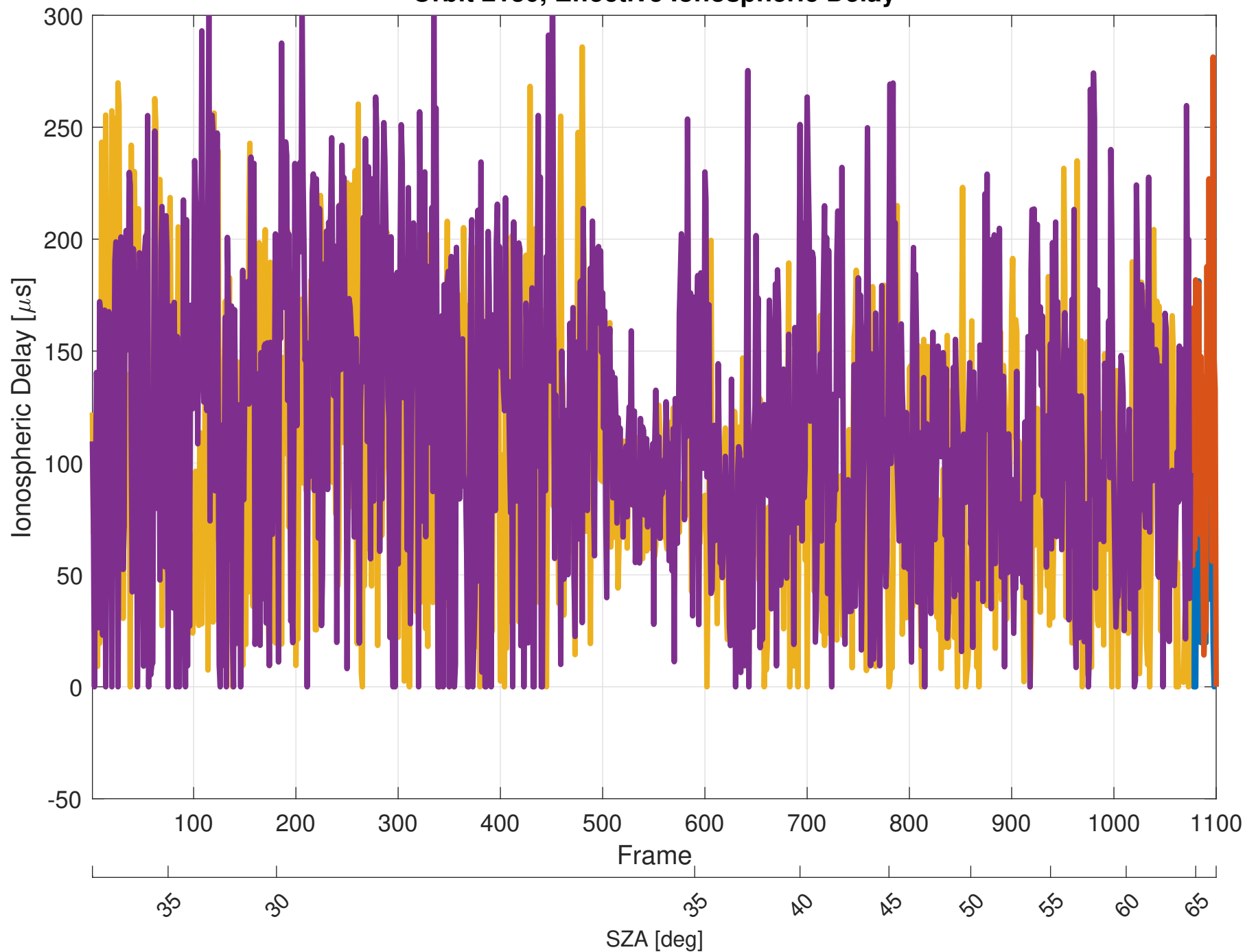
Orbit 2130, Effective Ionospheric Delay
