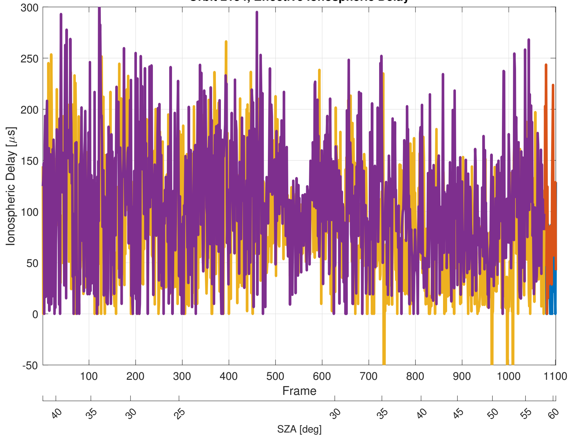
Orbit 2154, Effective Ionospheric Delay
