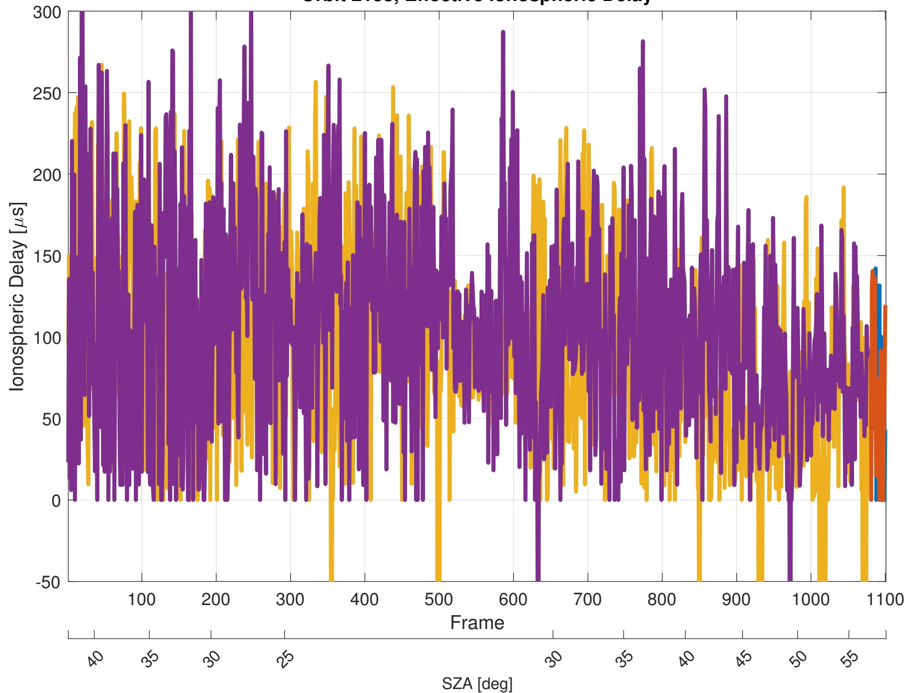
Orbit 2158, Effective Ionospheric Delay
