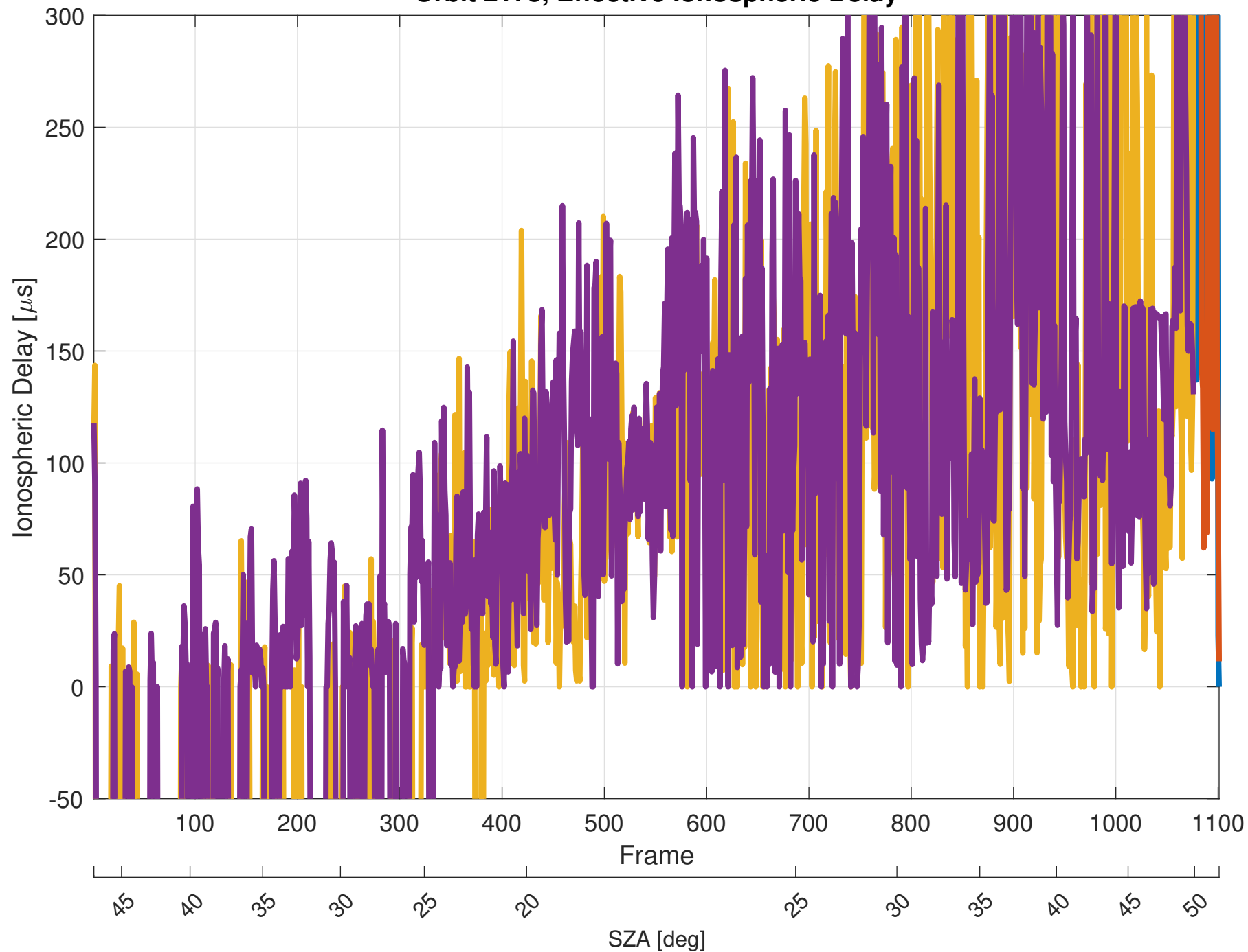
Orbit 2178, Effective Ionospheric Delay
