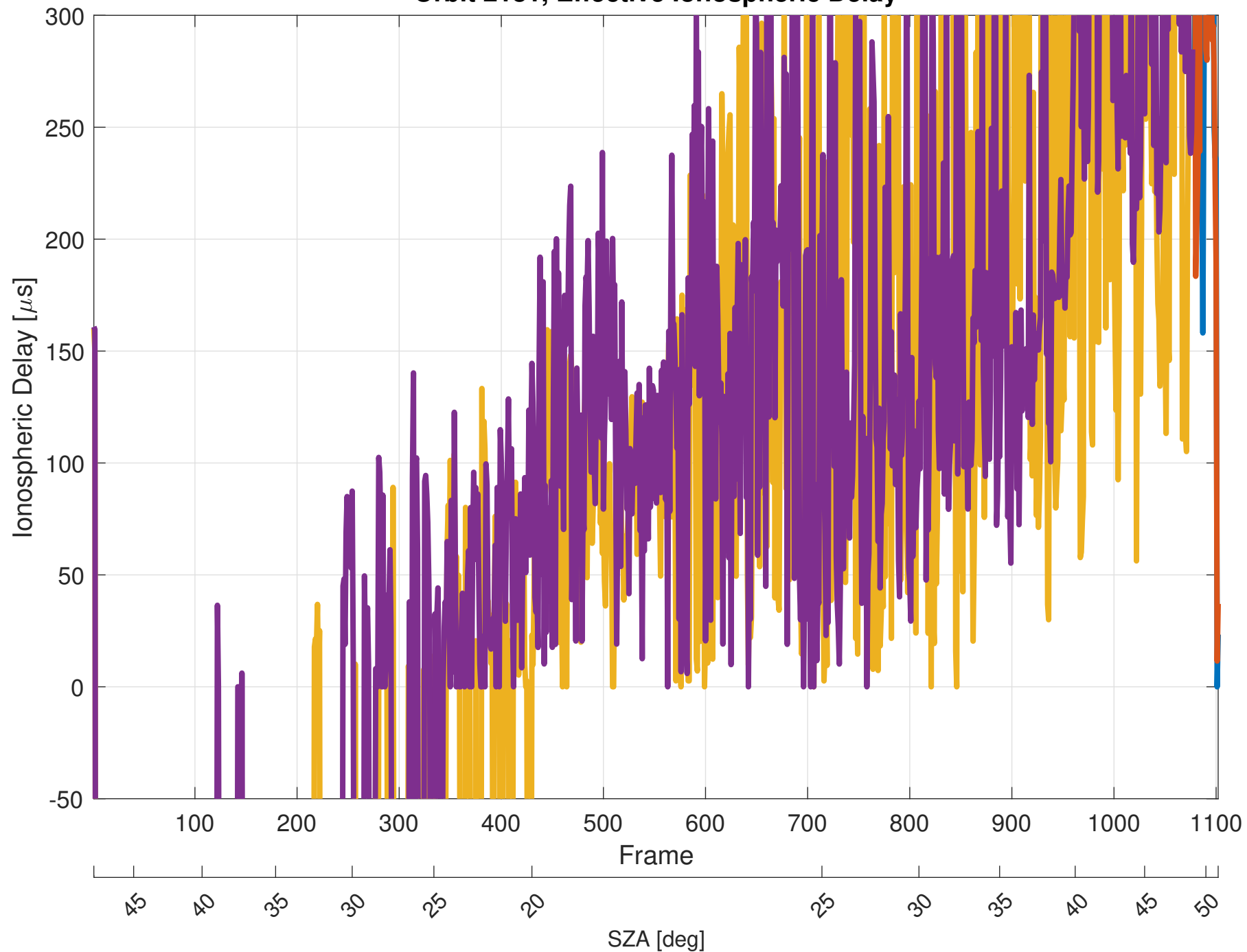
Orbit 2181, Effective Ionospheric Delay
