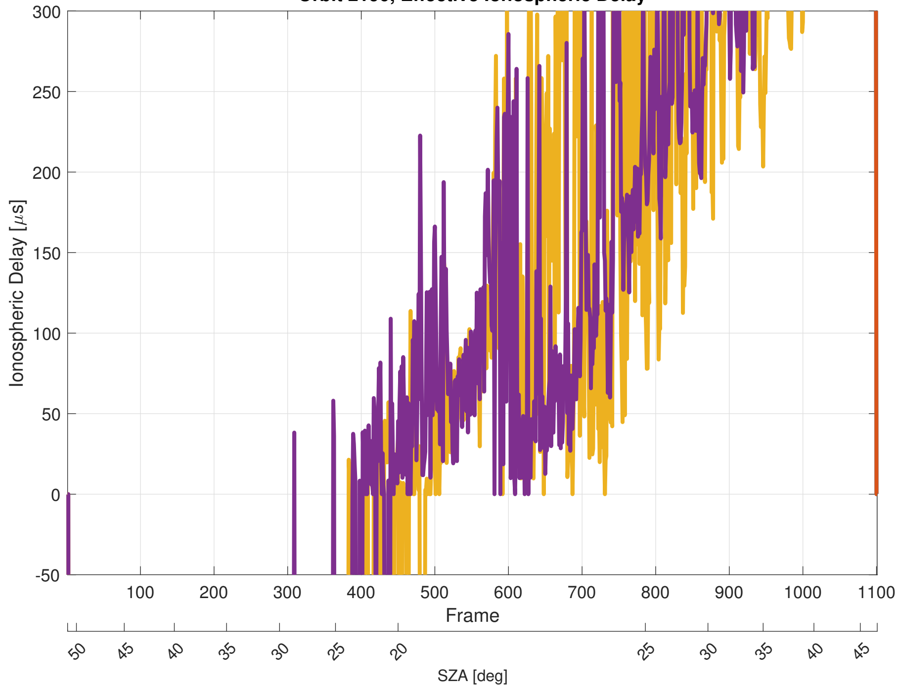
Orbit 2190, Effective Ionospheric Delay
