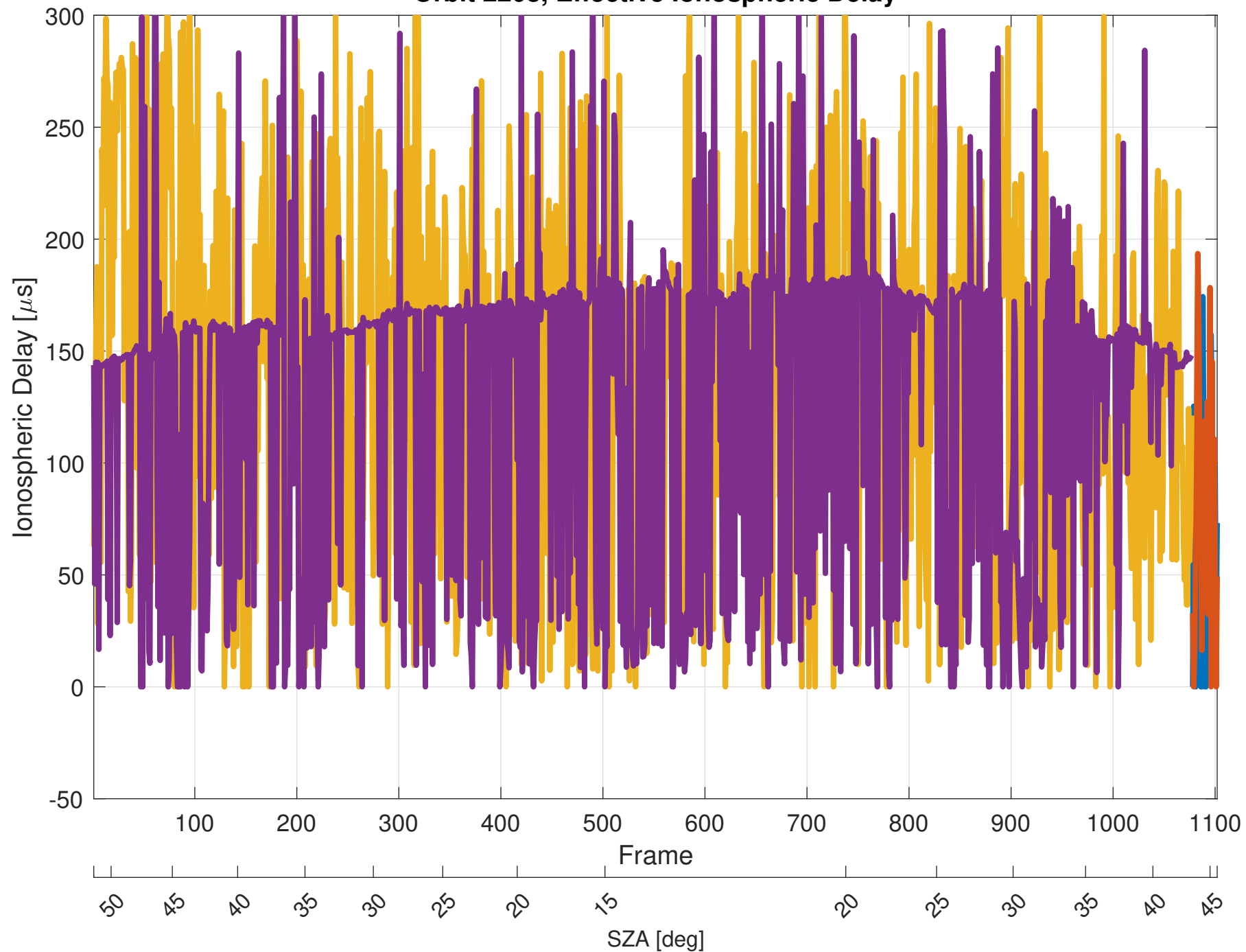
Orbit 2208, Effective Ionospheric Delay
