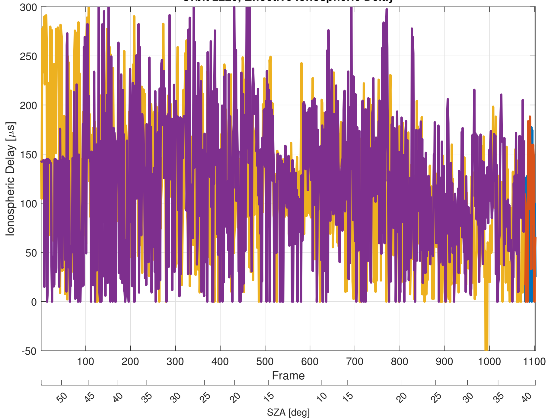
Orbit 2220, Effective Ionospheric Delay
