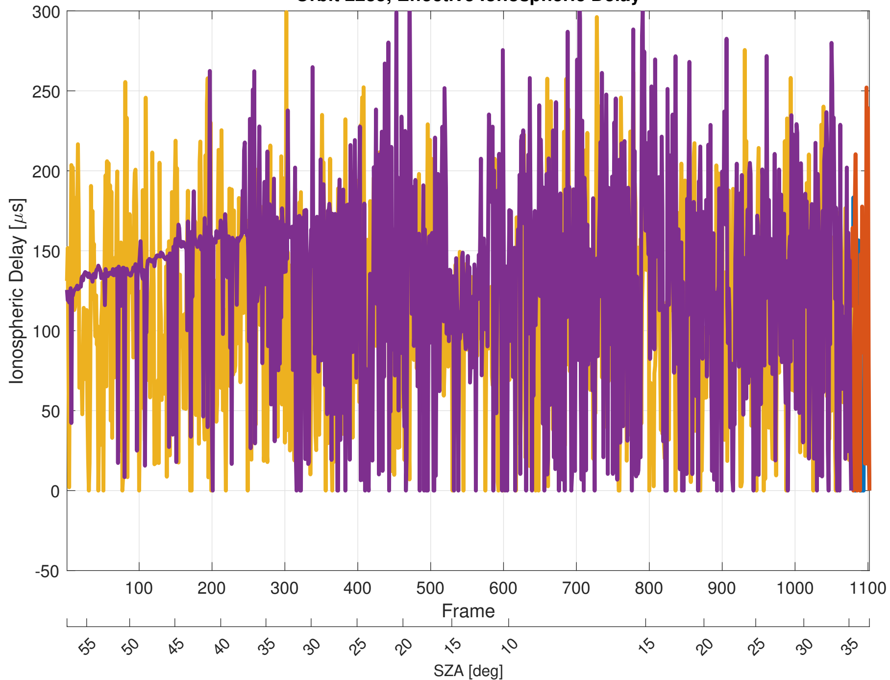
Orbit 2235, Effective Ionospheric Delay
