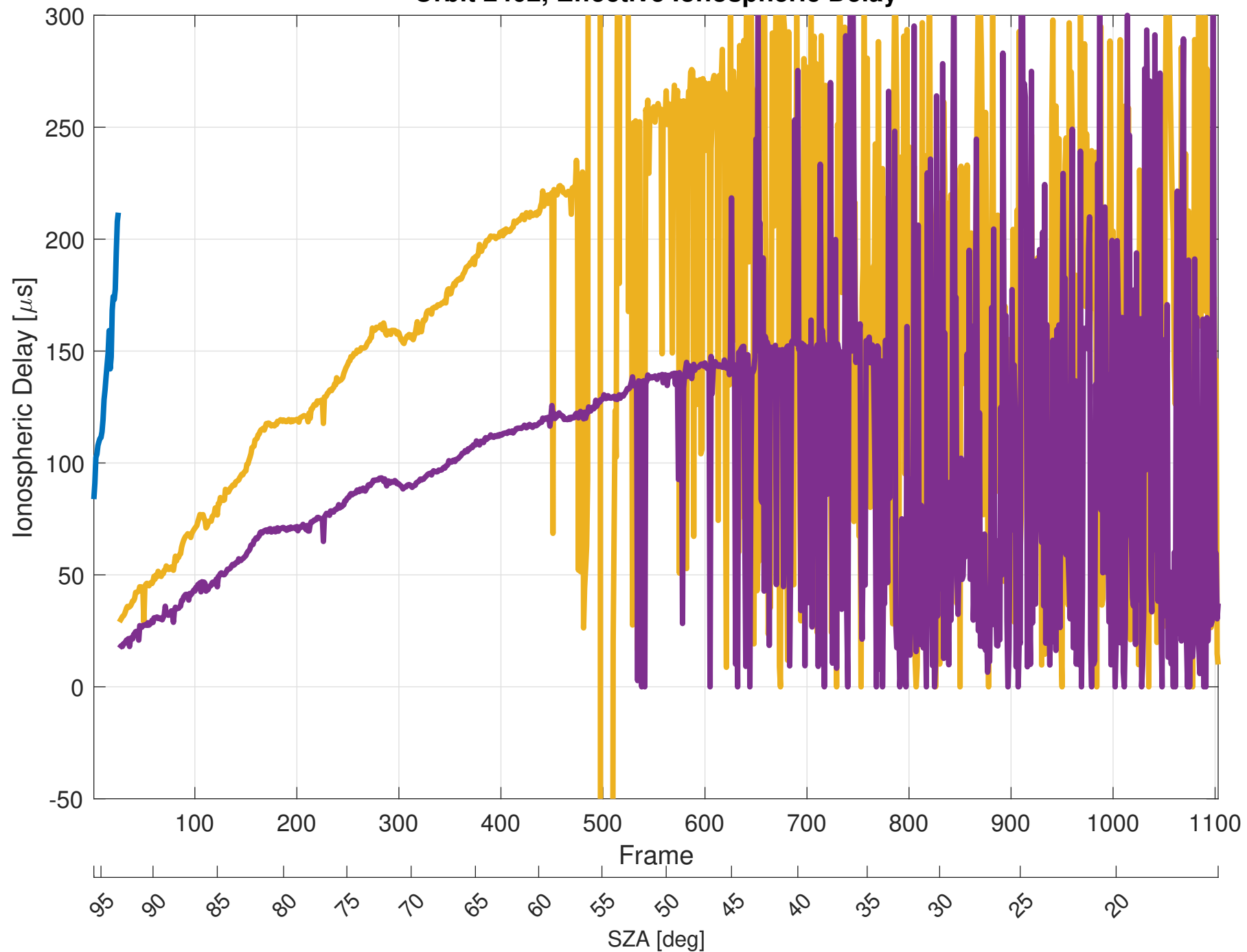
Orbit 2402, Effective Ionospheric Delay
