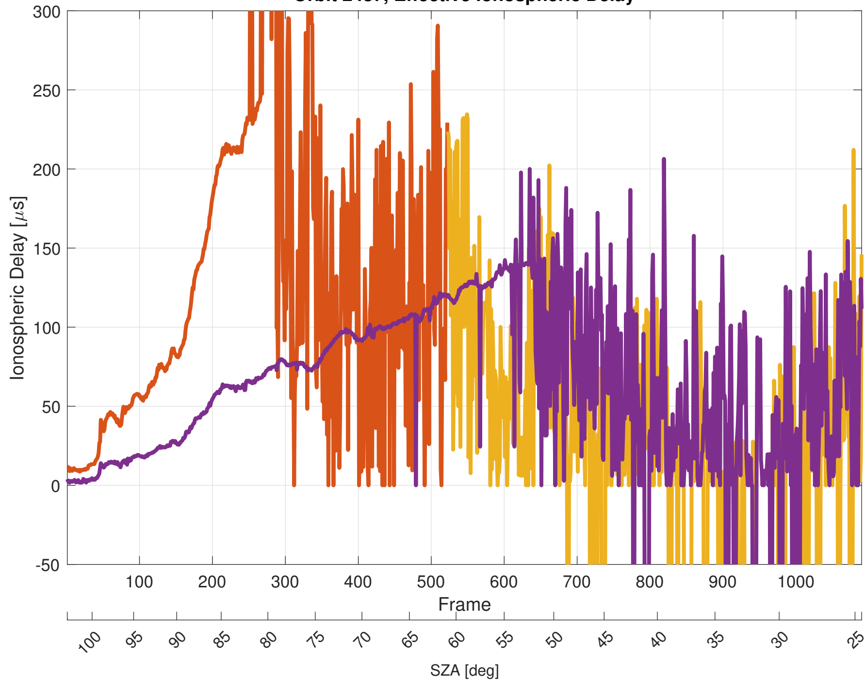
Orbit 2437, Effective Ionospheric Delay
