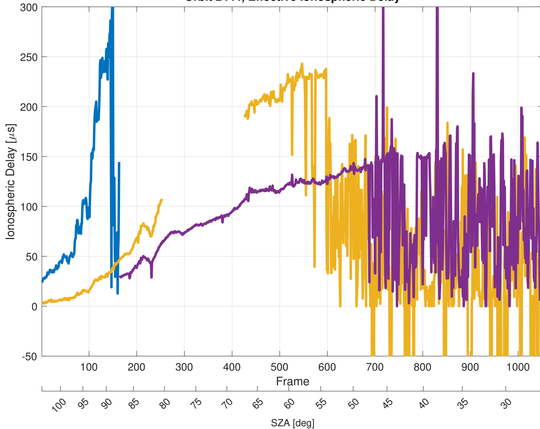
Orbit 2444, Effective Ionospheric Delay
