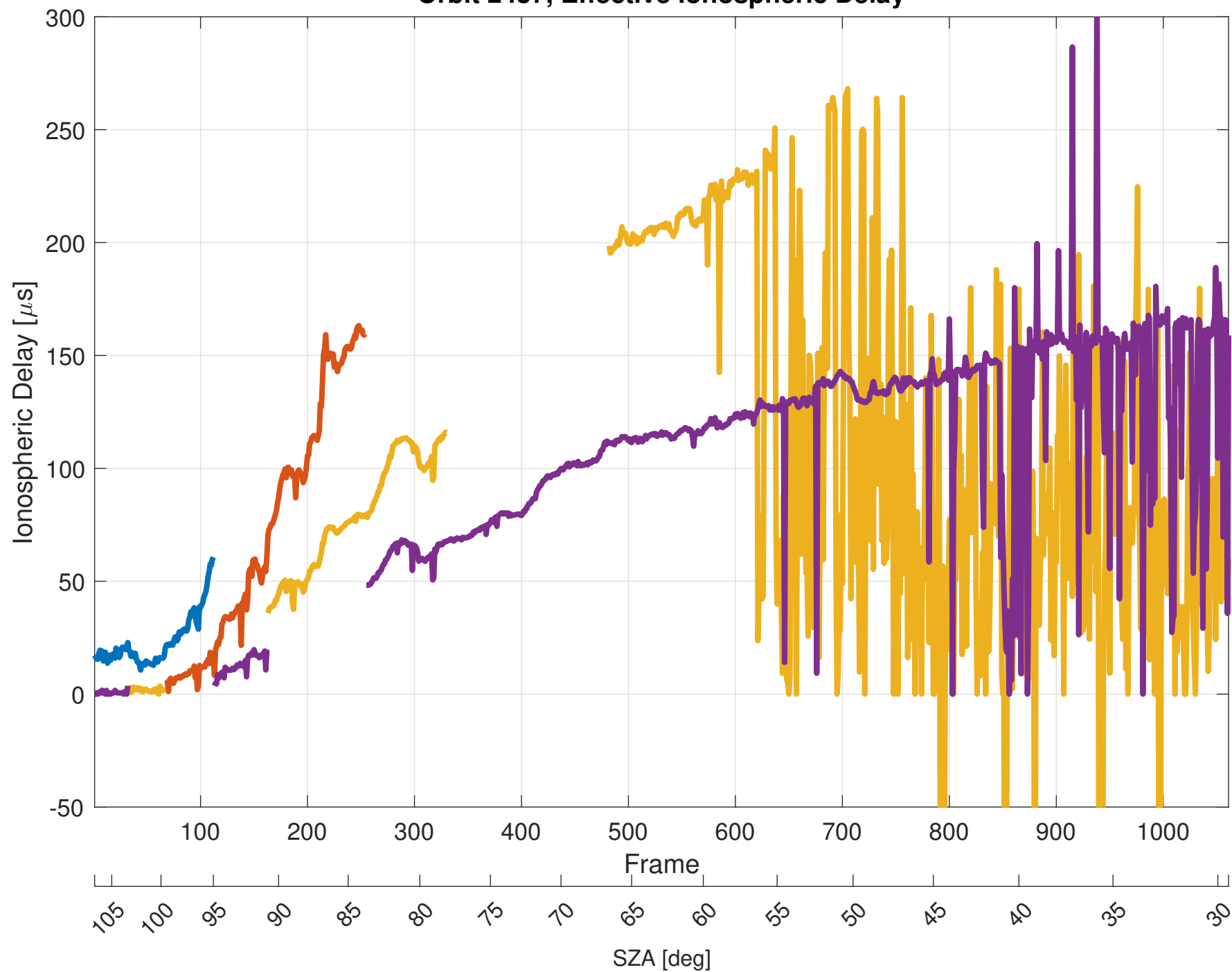
Orbit 2457, Effective Ionospheric Delay
