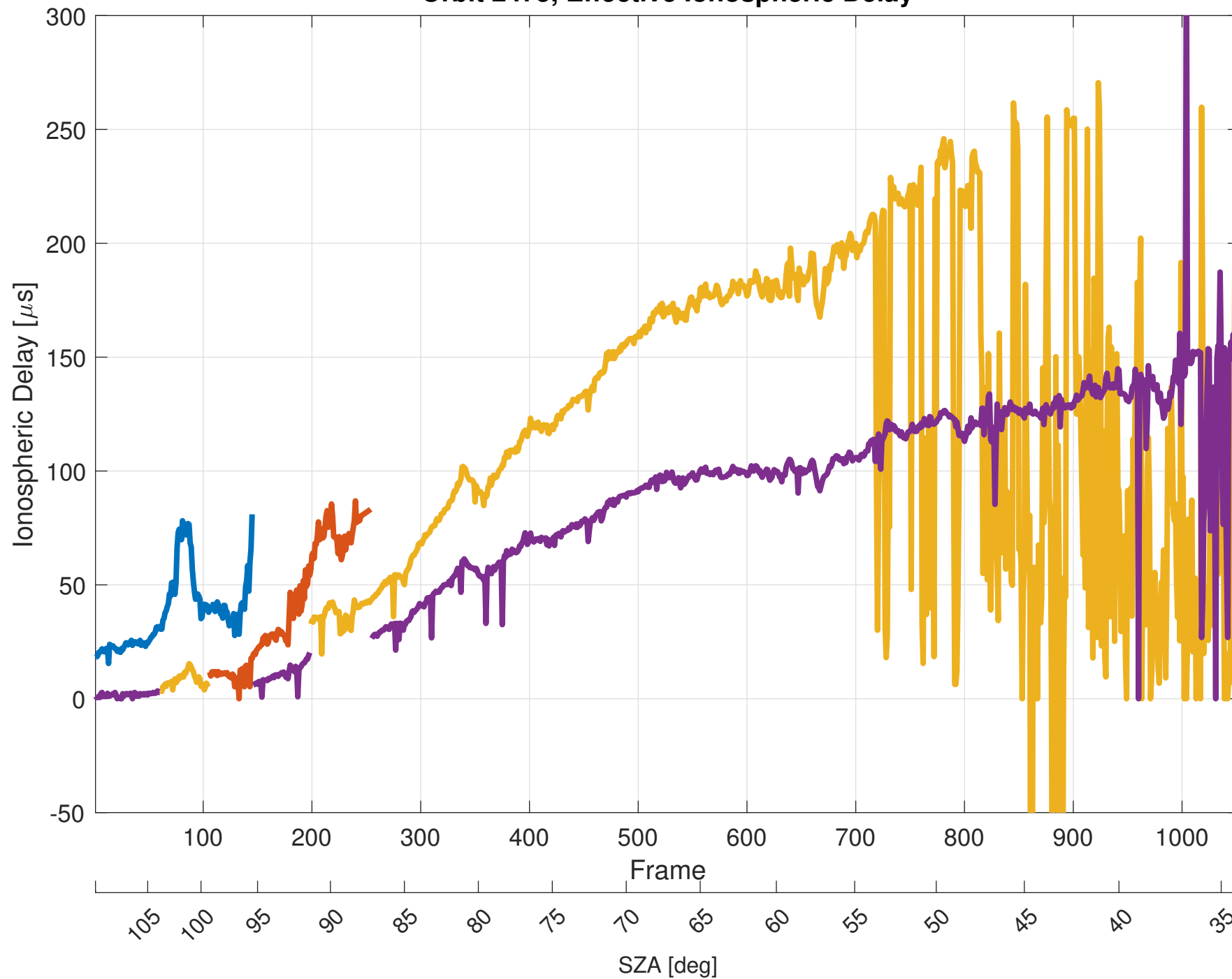
Orbit 2475, Effective Ionospheric Delay
