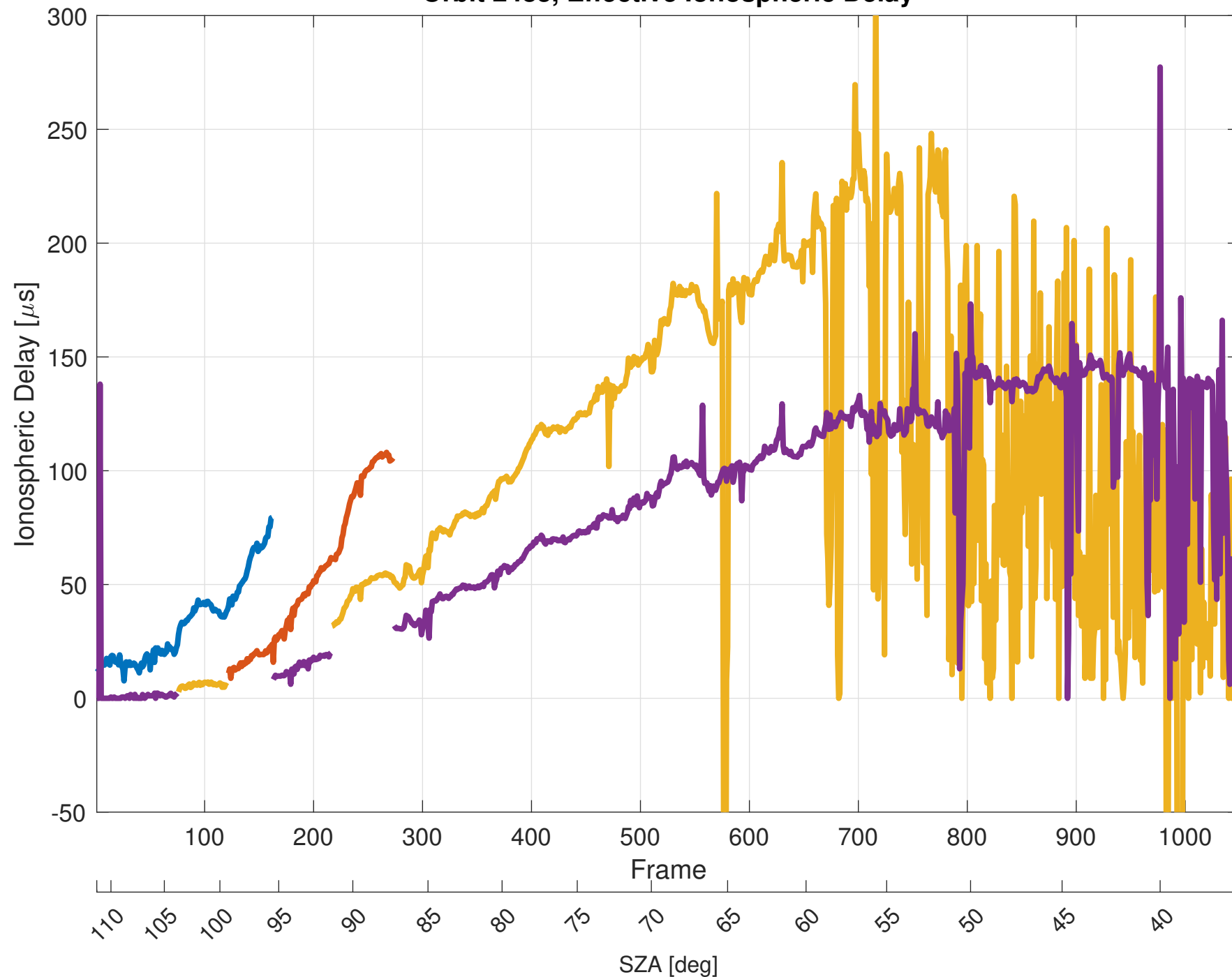
Orbit 2483, Effective Ionospheric Delay
