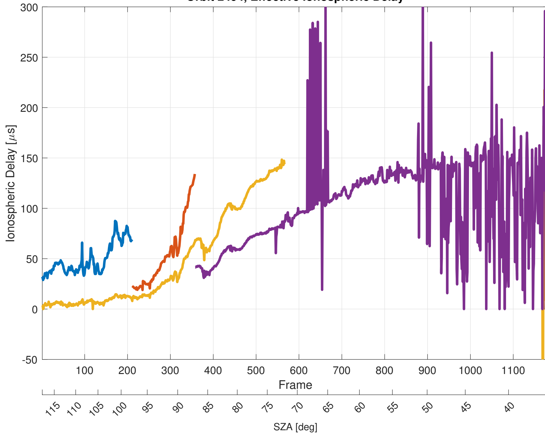
Orbit 2494, Effective Ionospheric Delay
