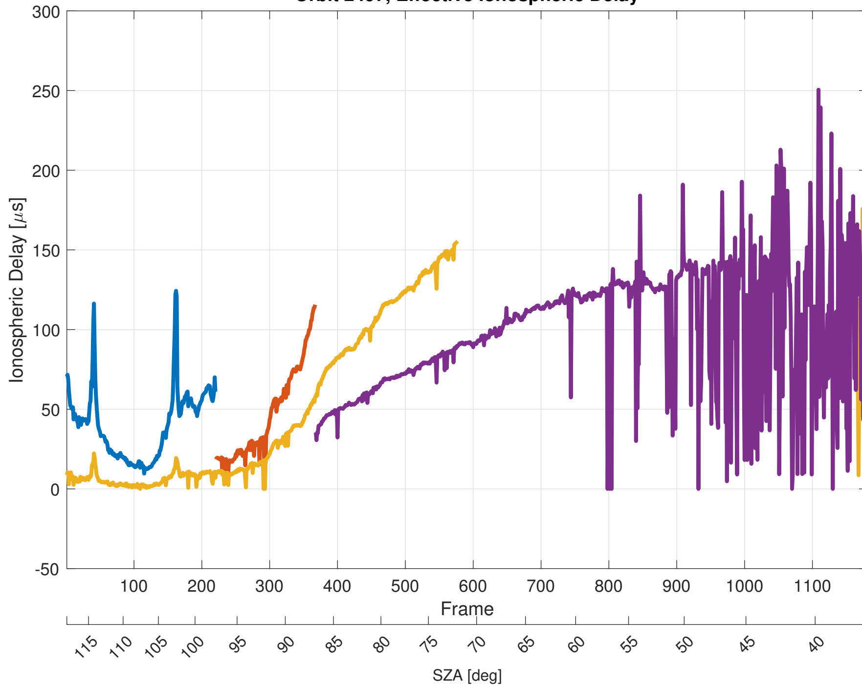
Orbit 2497, Effective Ionospheric Delay
