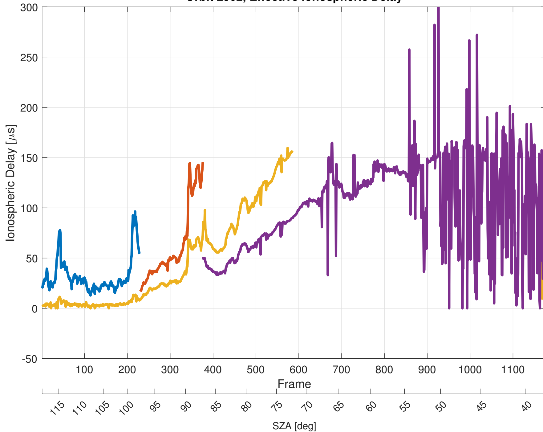
Orbit 2502, Effective Ionospheric Delay
