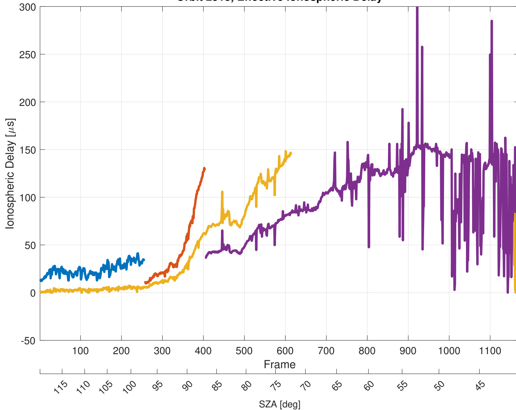
Orbit 2513, Effective Ionospheric Delay
