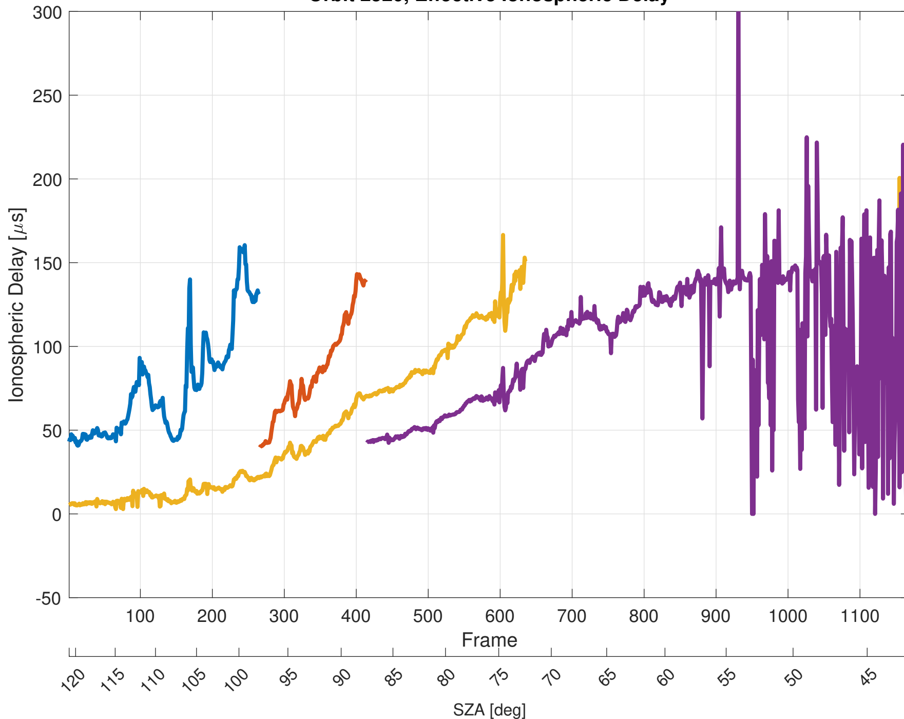
Orbit 2520, Effective Ionospheric Delay
