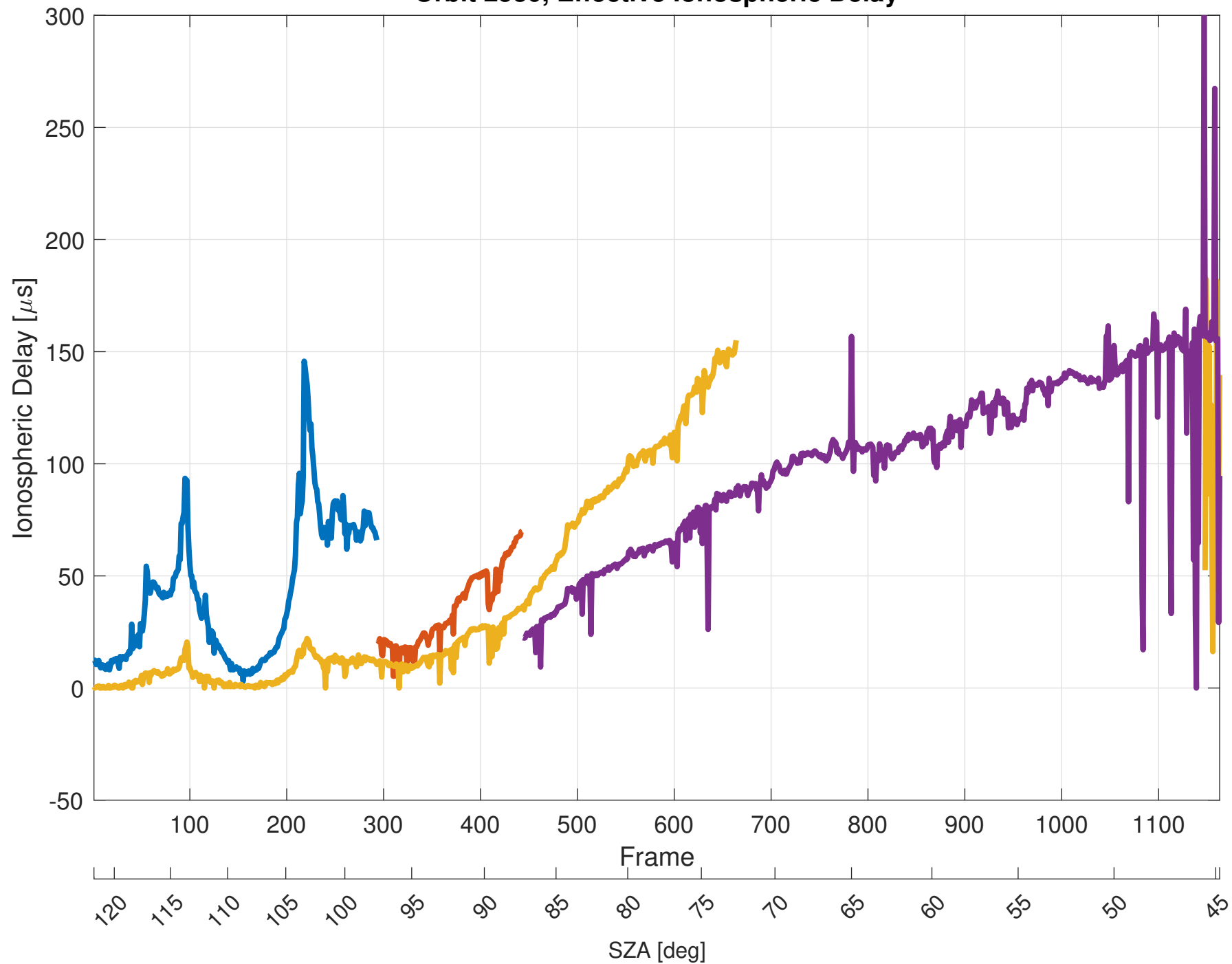
Orbit 2530, Effective Ionospheric Delay
