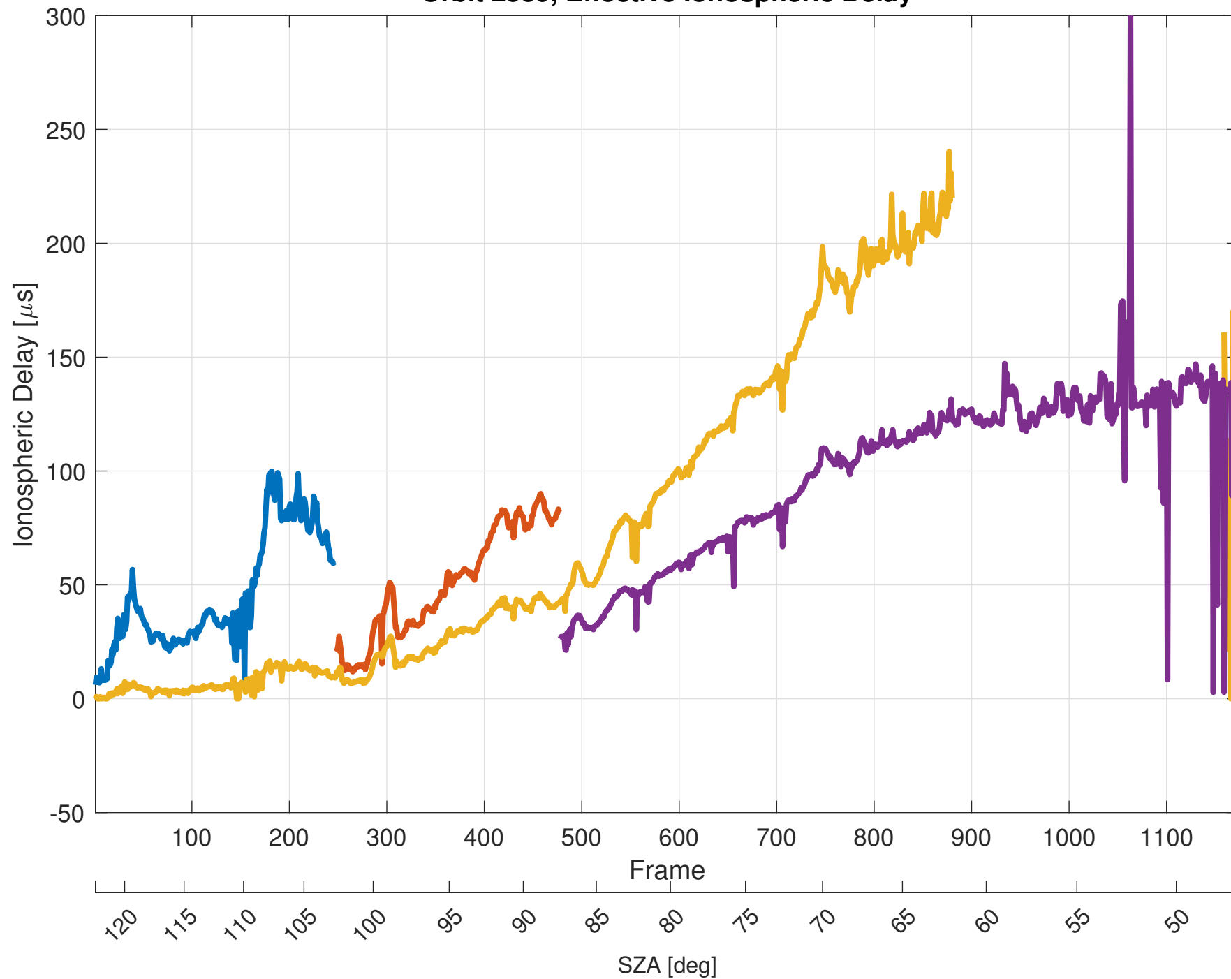
Orbit 2539, Effective Ionospheric Delay
