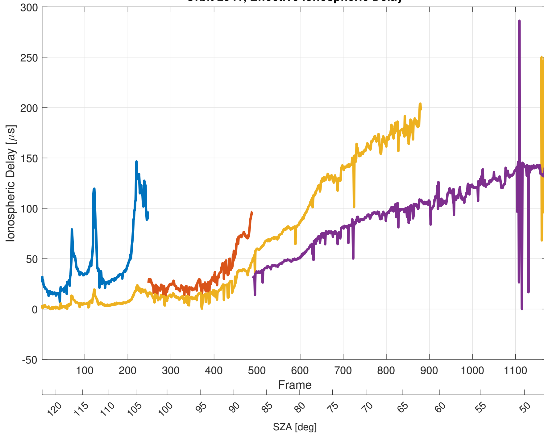
Orbit 2541, Effective Ionospheric Delay
