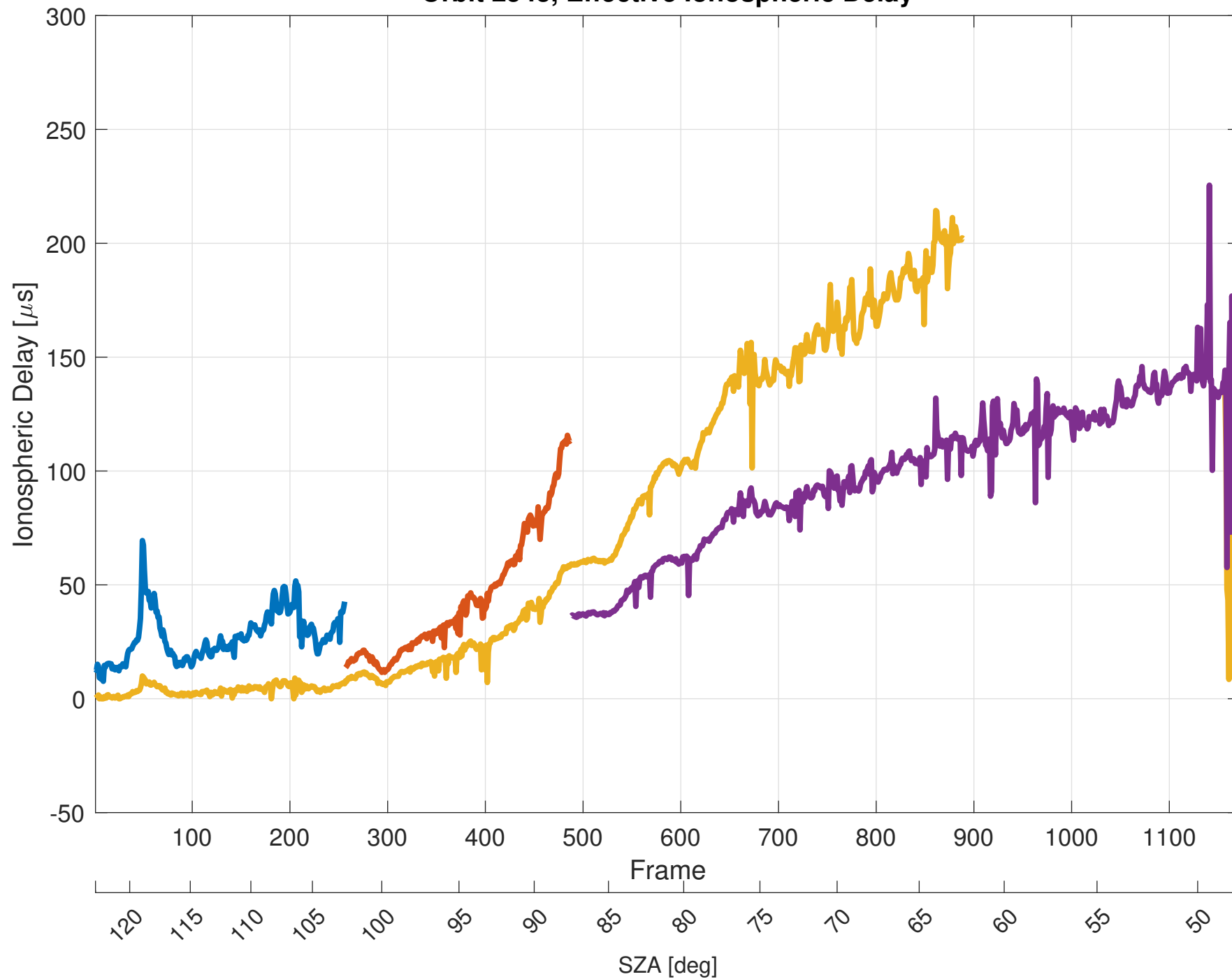
Orbit 2543, Effective Ionospheric Delay
