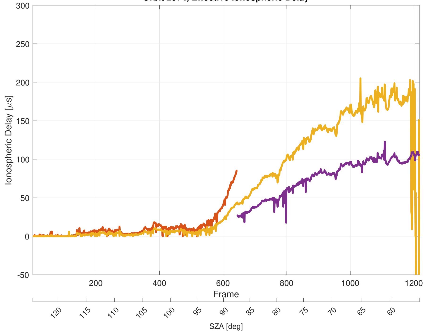
Orbit 2574, Effective Ionospheric Delay
