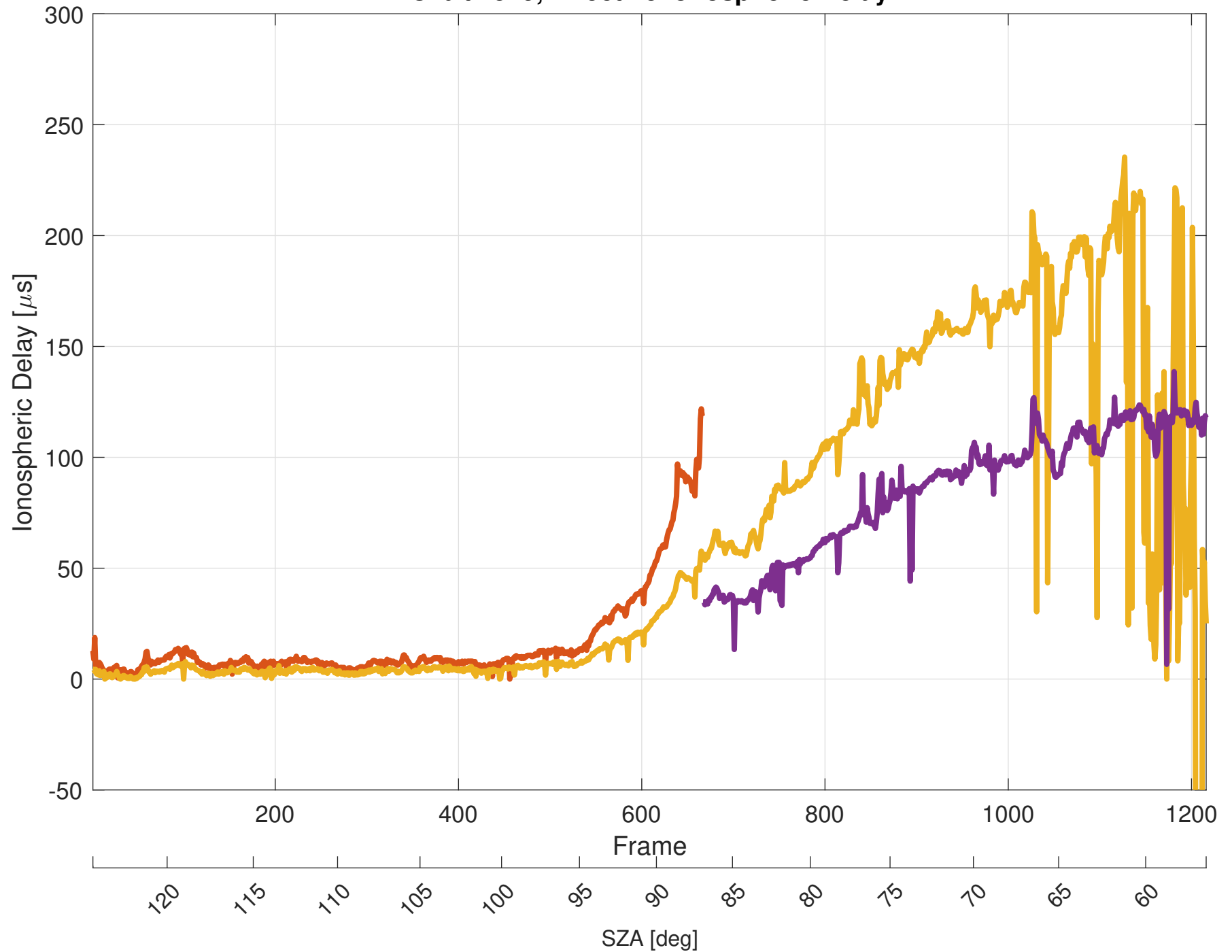
Orbit 2579, Effective Ionospheric Delay
