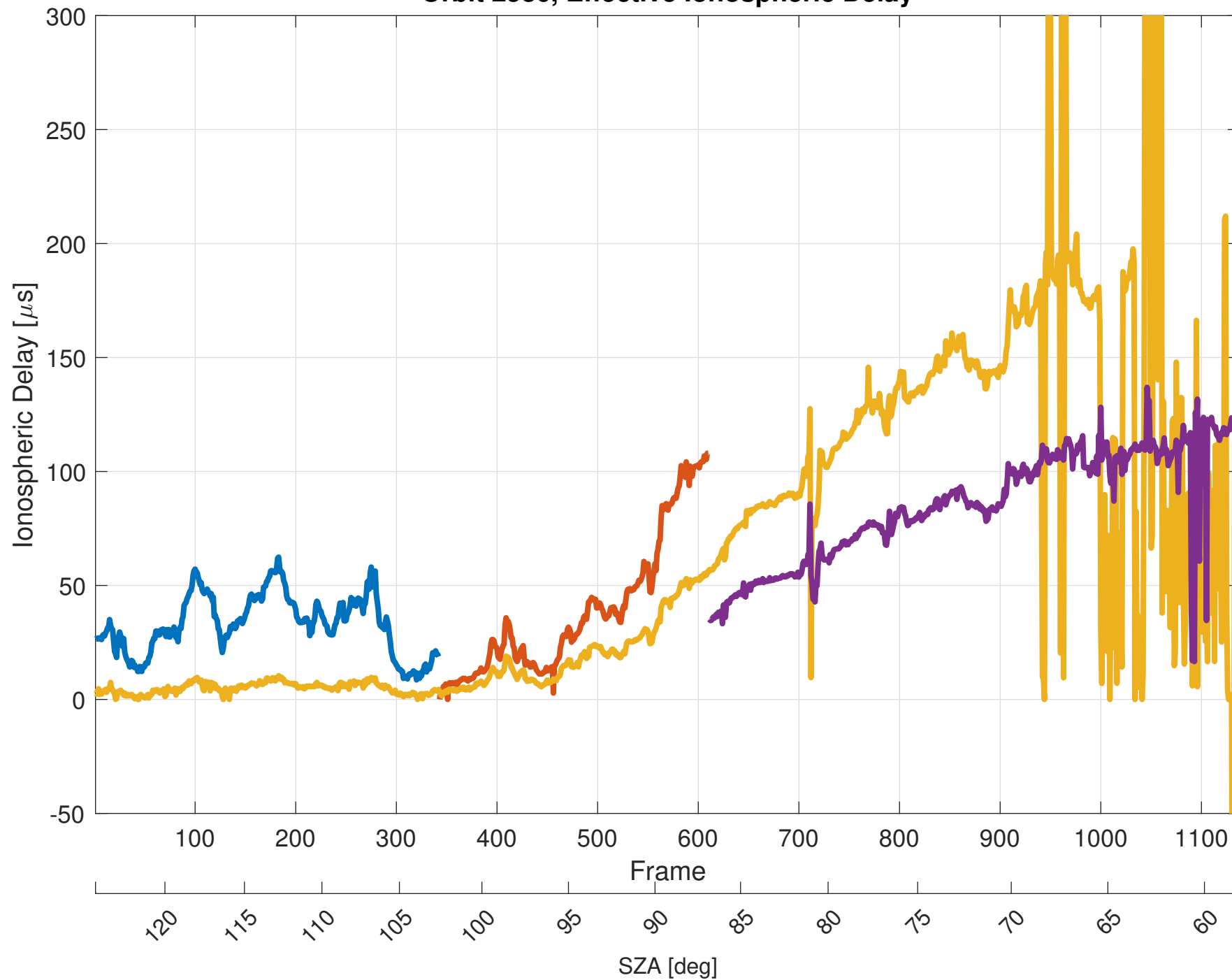
Orbit 2586, Effective Ionospheric Delay
