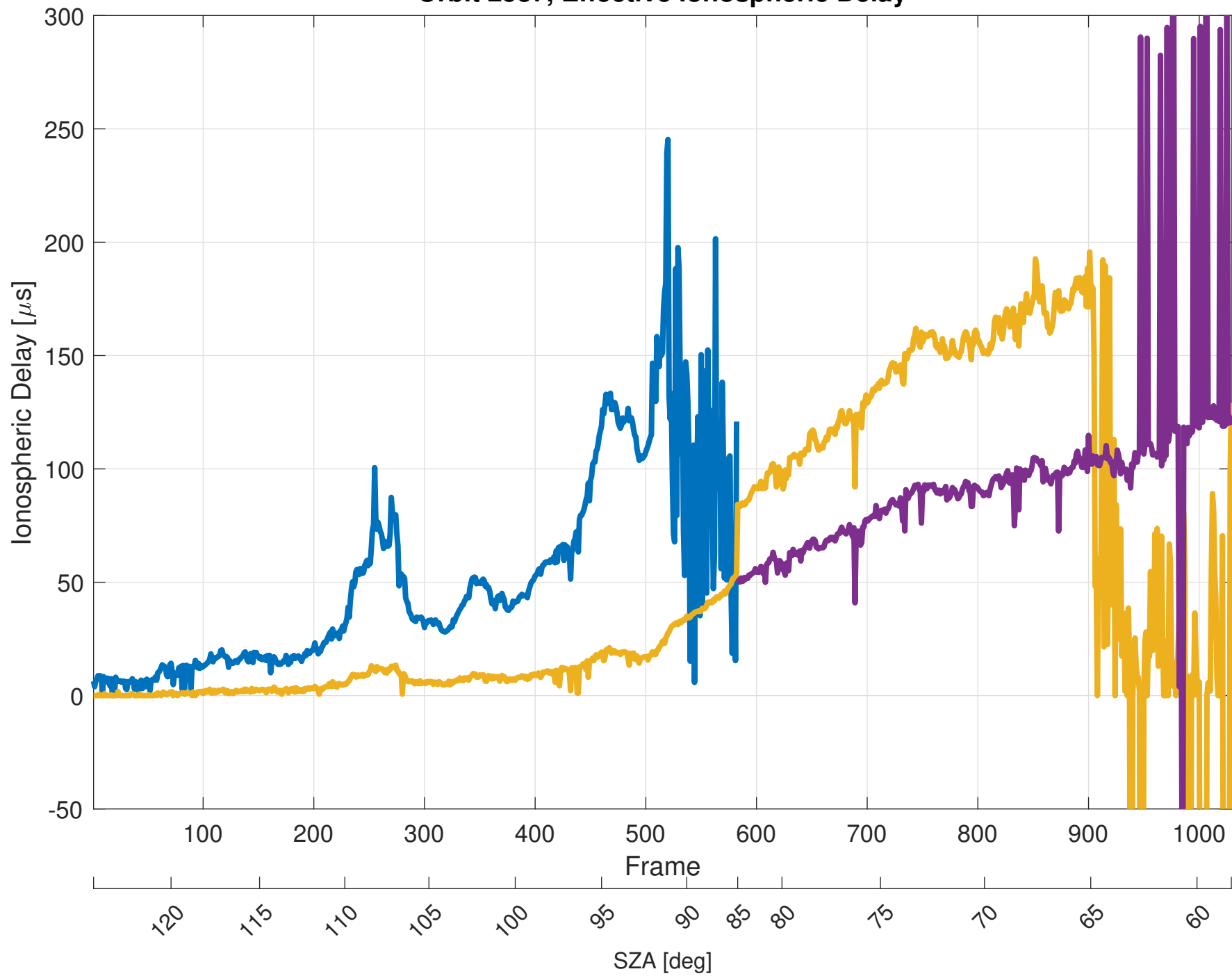
Orbit 2587, Effective Ionospheric Delay
