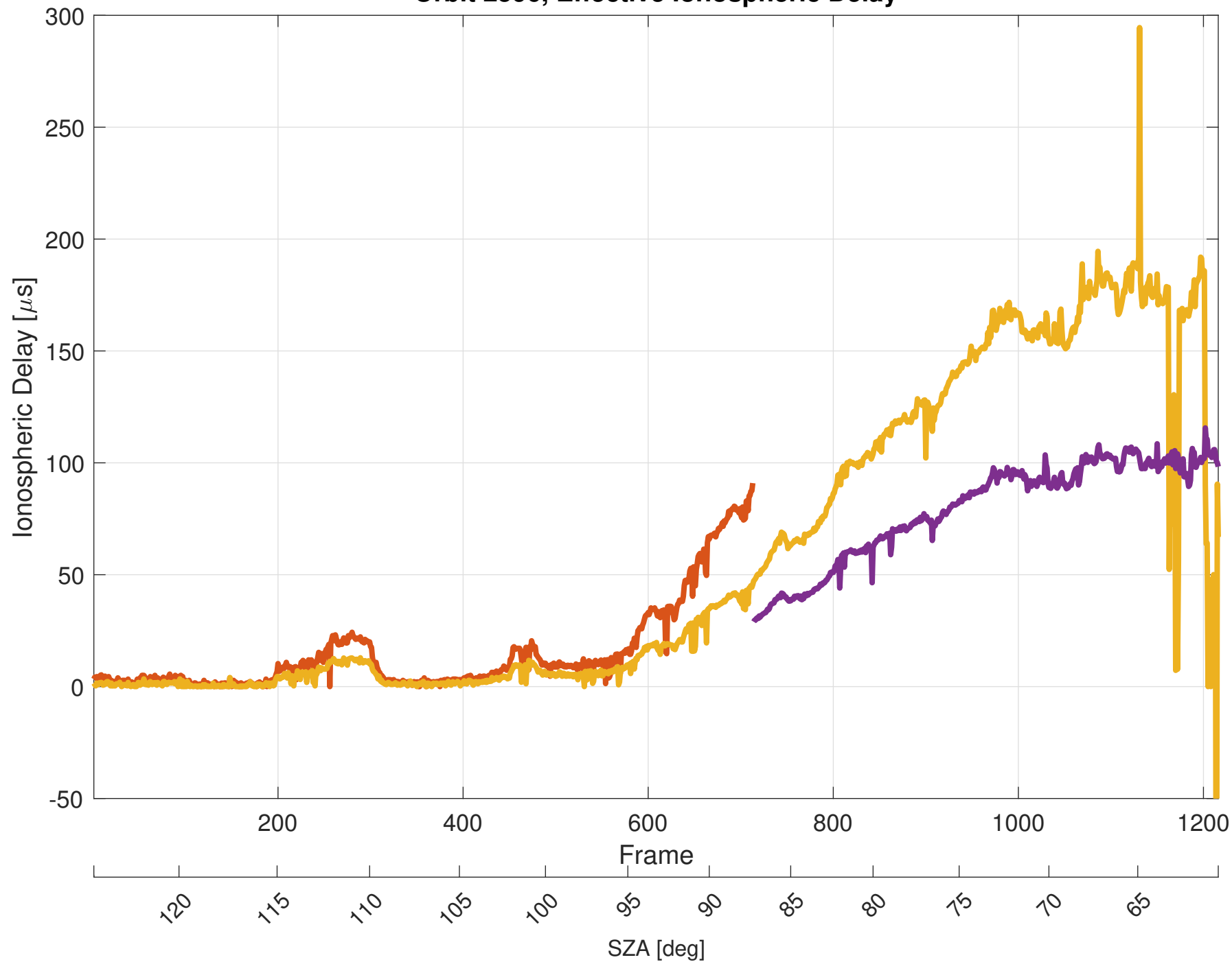
Orbit 2596, Effective Ionospheric Delay
