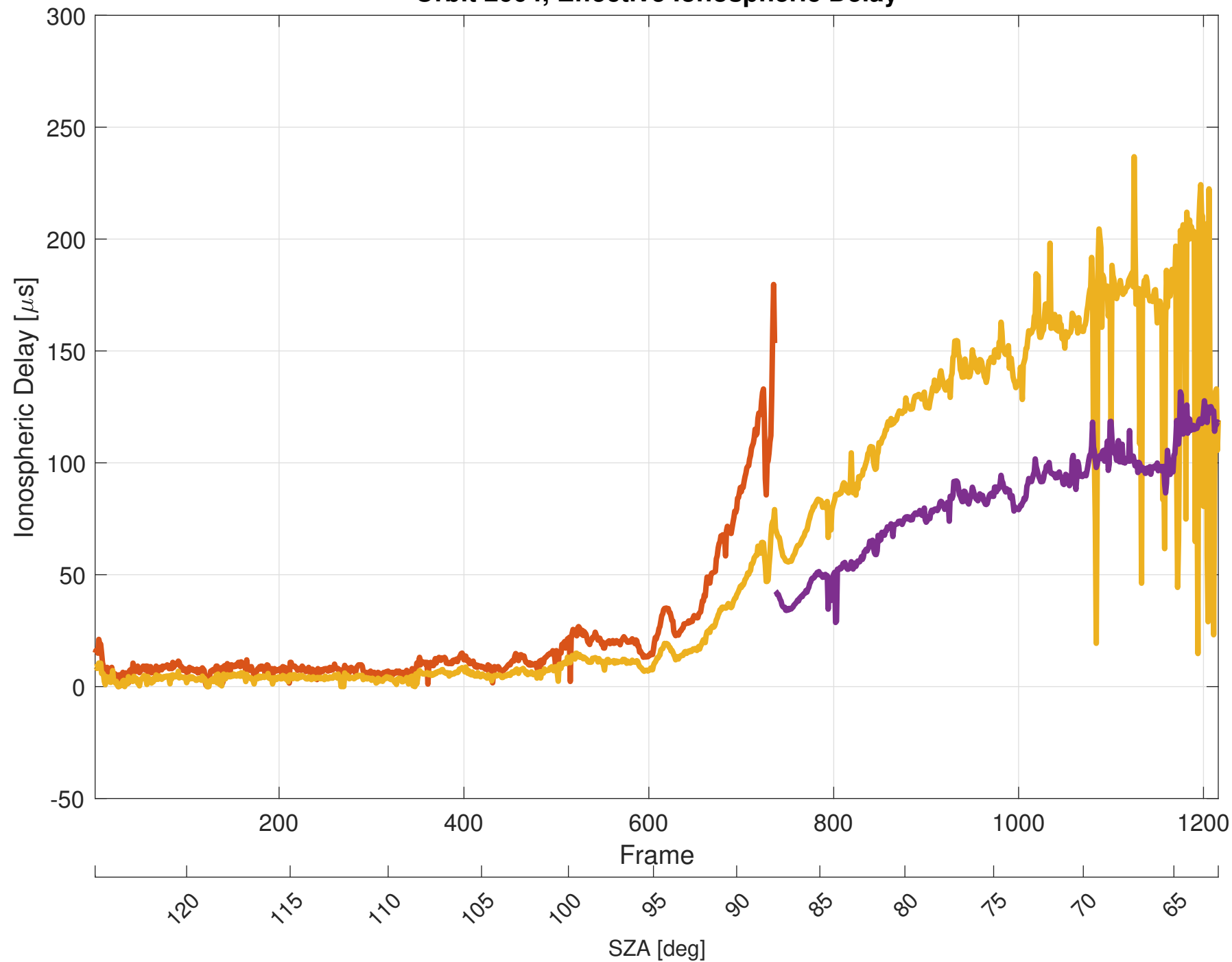
Orbit 2604, Effective Ionospheric Delay
