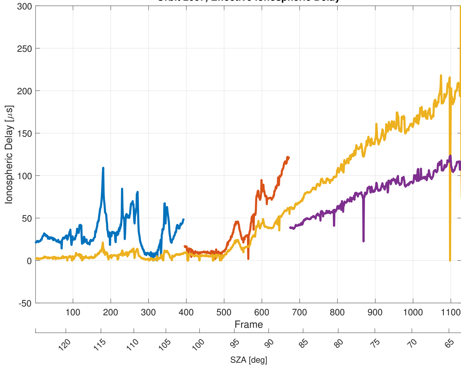
Orbit 2607, Effective Ionospheric Delay
