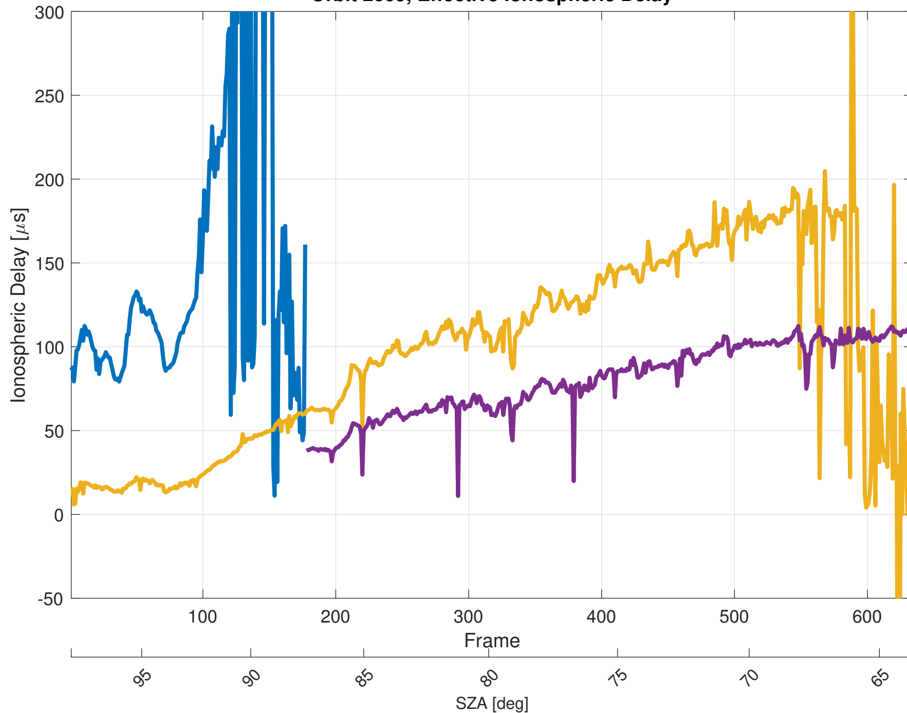
Orbit 2609, Effective Ionospheric Delay
