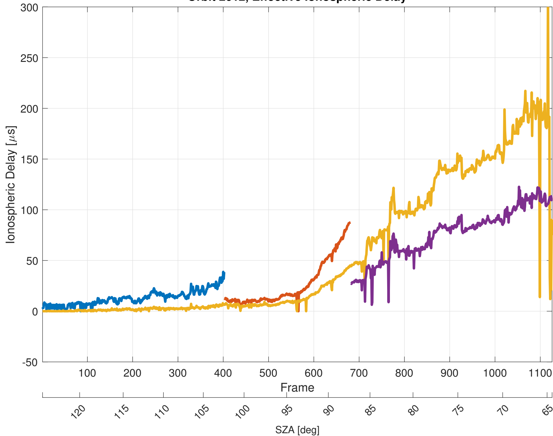
Orbit 2612, Effective Ionospheric Delay
