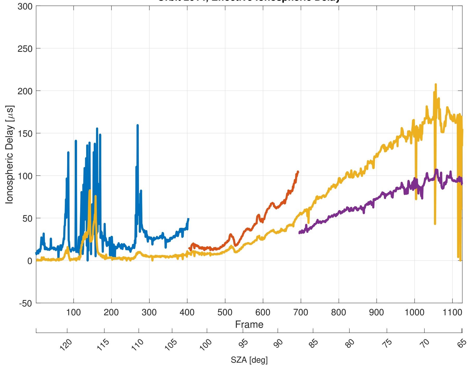
Orbit 2614, Effective Ionospheric Delay
