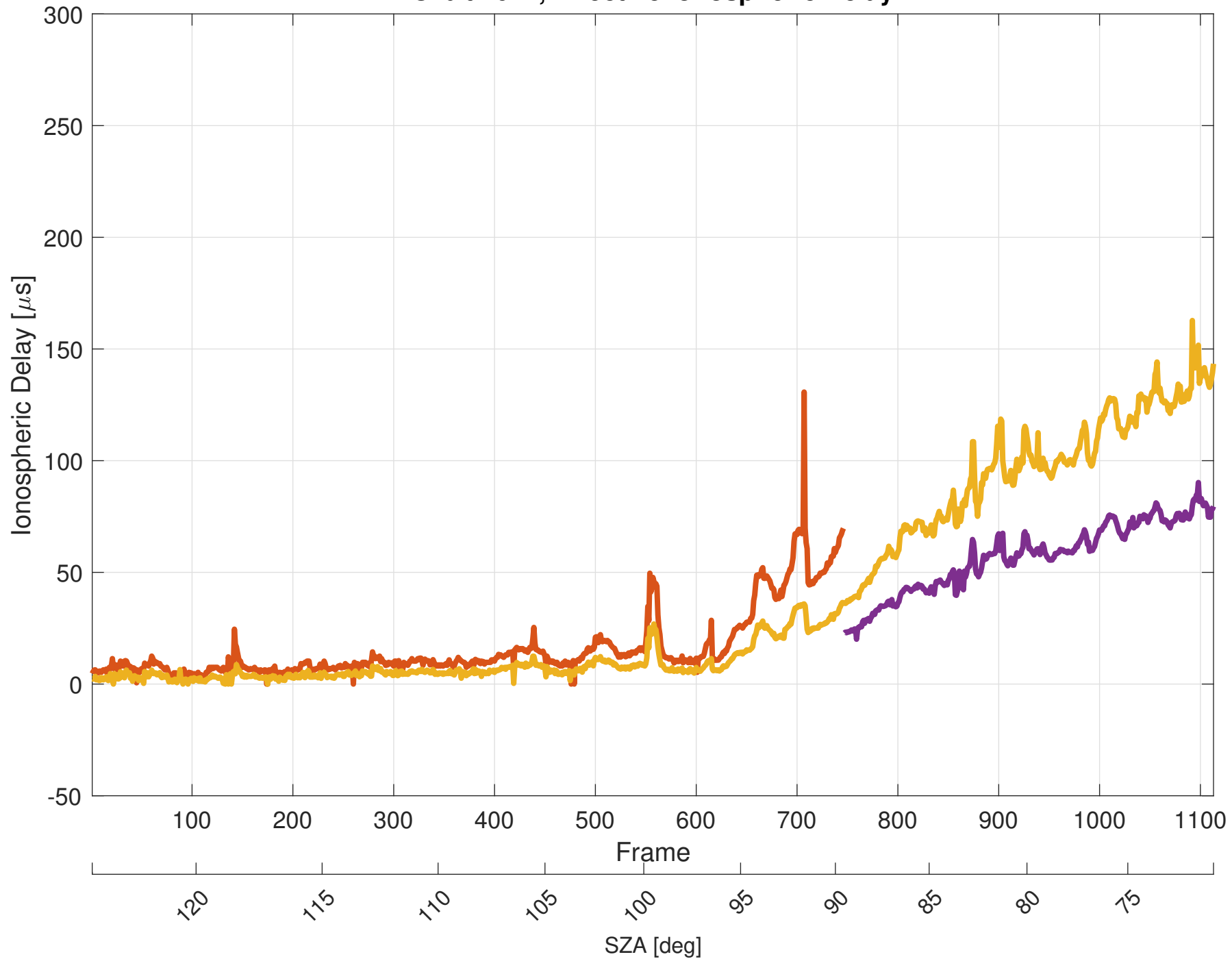
Orbit 2617, Effective Ionospheric Delay
