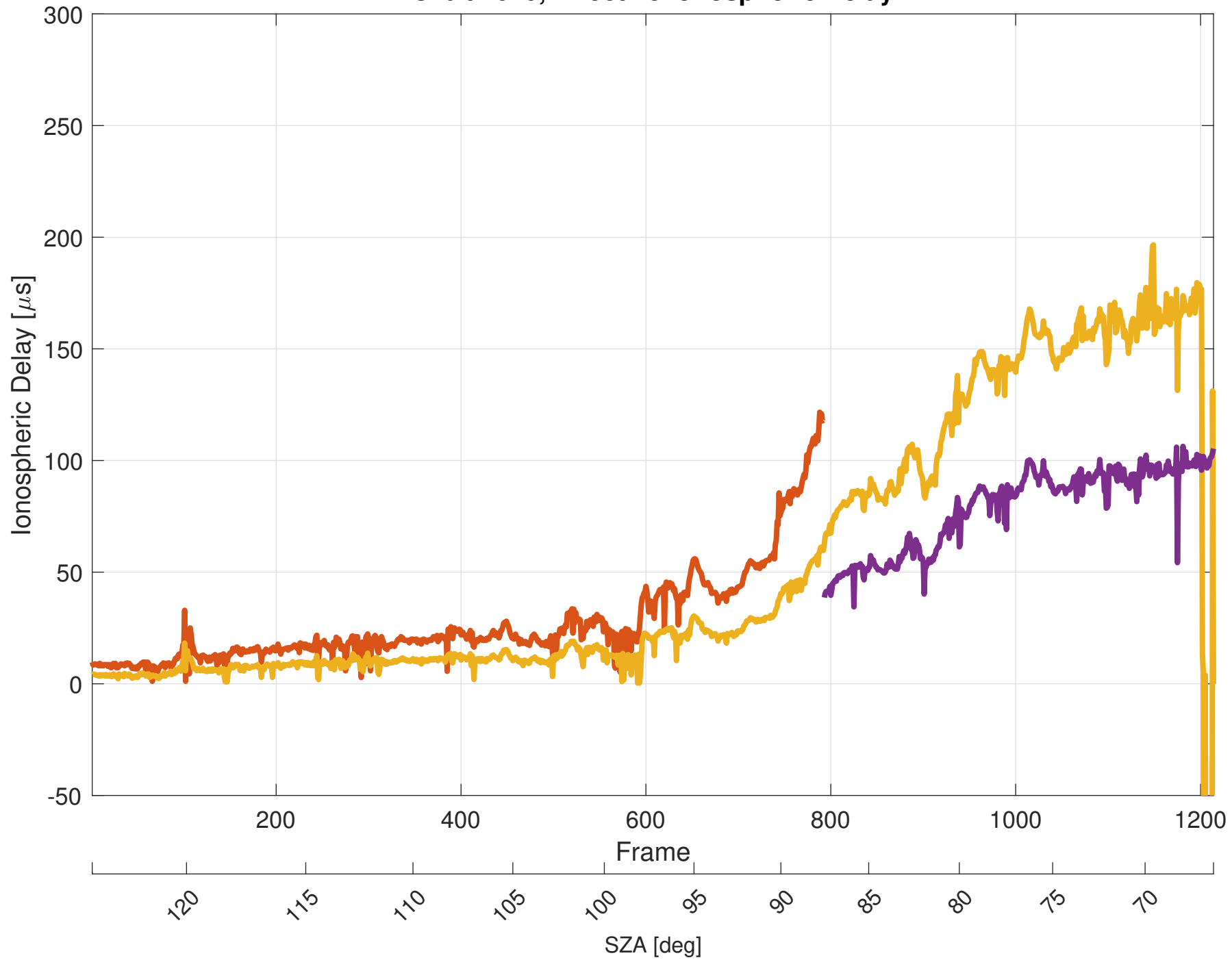
Orbit 2620, Effective Ionospheric Delay
