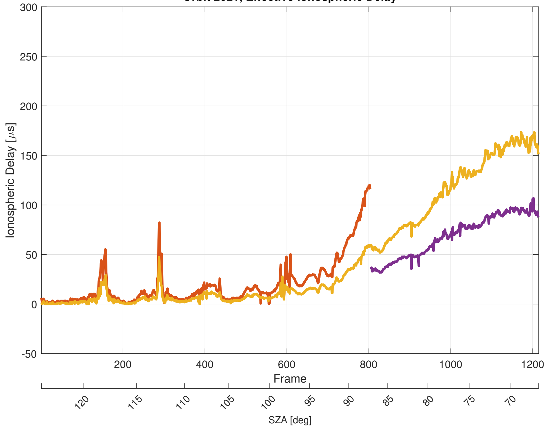
Orbit 2621, Effective Ionospheric Delay
