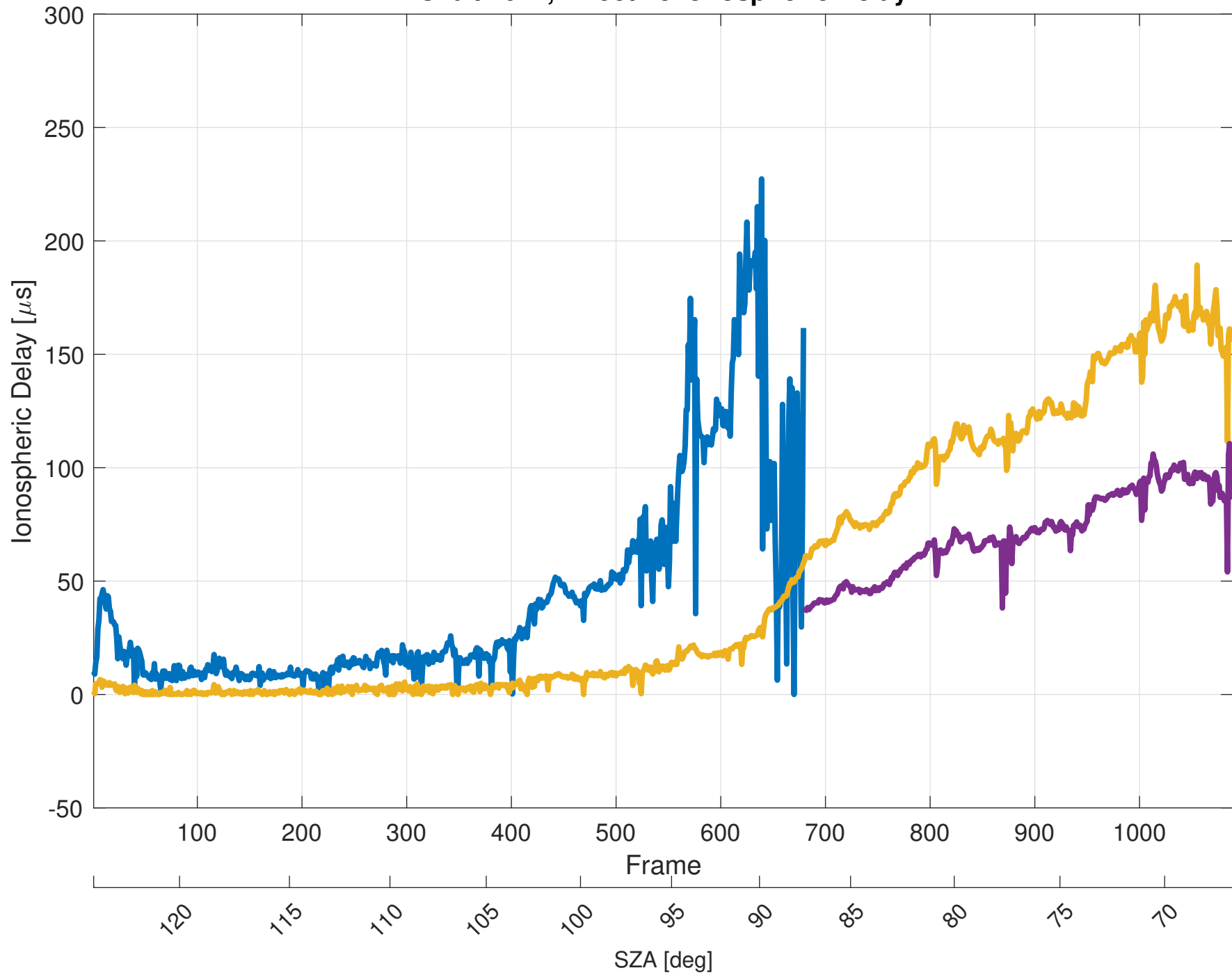
Orbit 2622, Effective Ionospheric Delay
